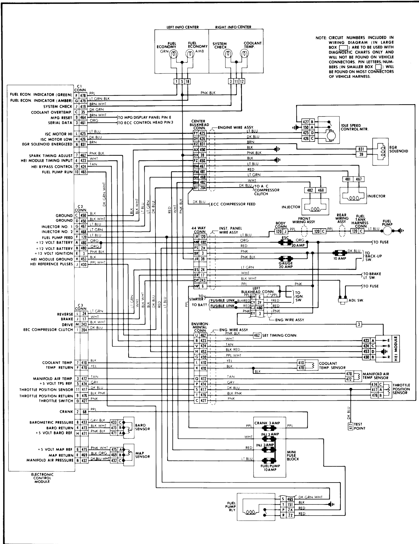
Digital Electronic Fuel Injection (DEFI) Wiring Diagram for General Motors
