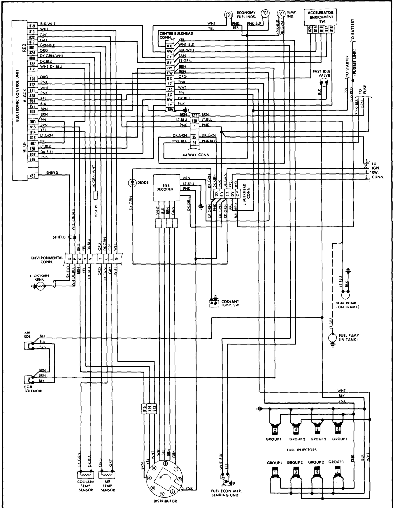
Electronic Fuel Injection (EFI) Wiring Diagram for General Motors
