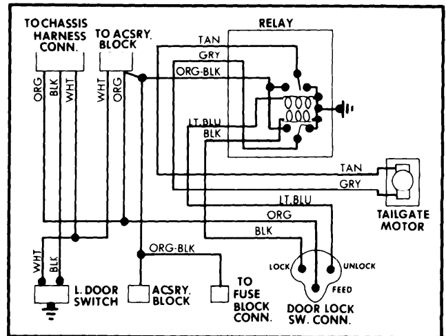
Relay System Electric Door Locks Wiring Diagram for Buick Station Wagon Tailgate Lock Only
