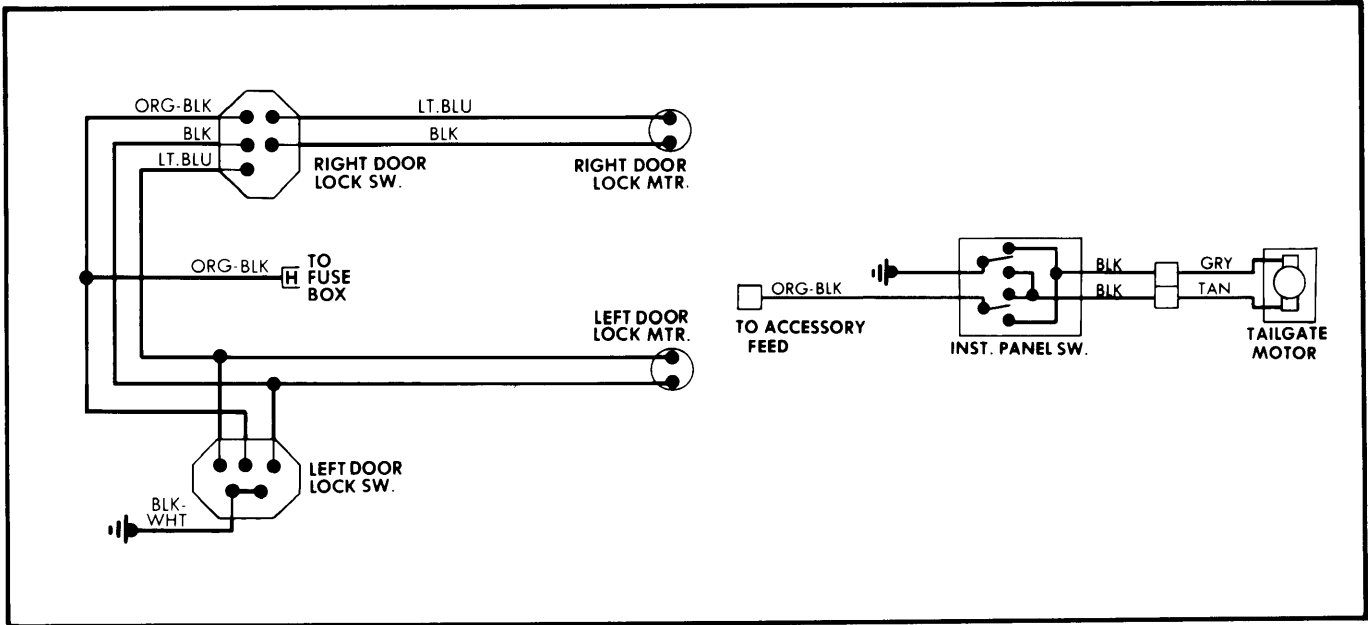
Polarity Switch System Door Locks Wiring Diagram for Camaro, Firebird and Station Wagons (Exc. Buick)
