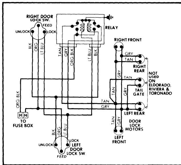
Relay System Electric Door Locks, Including Station Wagons with Both Door and Tailgate Locks, Wiring Diagram for General Motors
