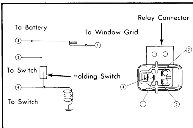
Heated Rear Window Relay Connections Wiring Diagram for Ford Motor Co. (Granada, Monarch, Pinto and Bobcat)
