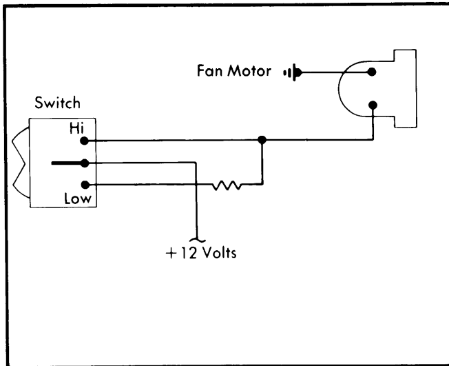
Rear Window Defogger Fan Circuit with Resistor or Resistance Wire in Circuit Wiring Diagram for General Motors
