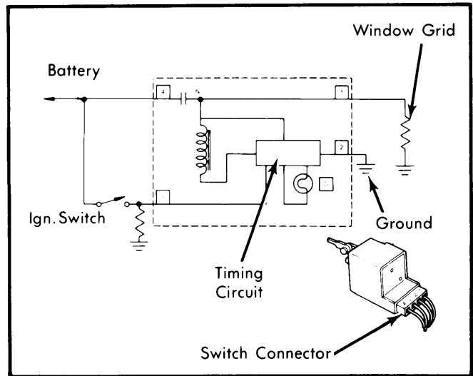
Heated Rear Window Wiring Diagram for Ford Motor Co. (Continental, Mark VI, Ford, Mercury, Thunderbird and Cougar XR-7)
