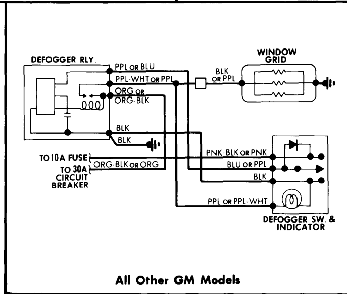
Electric Window Defogger Wiring Diagram for General Motors (All Models)
