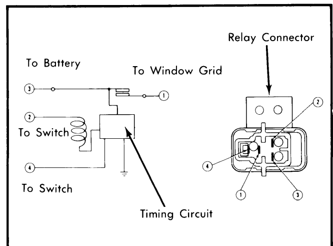
Heated Rear Window Relay Connections Wiring Diagram for Ford Motor Co. (Versailles, Fairmont and Zephyr)
