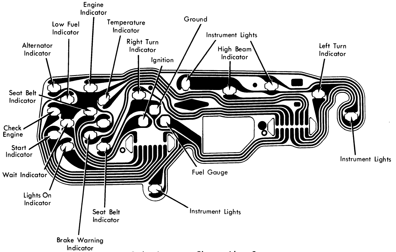
Cutlass Instrument Cluster without Gauges
