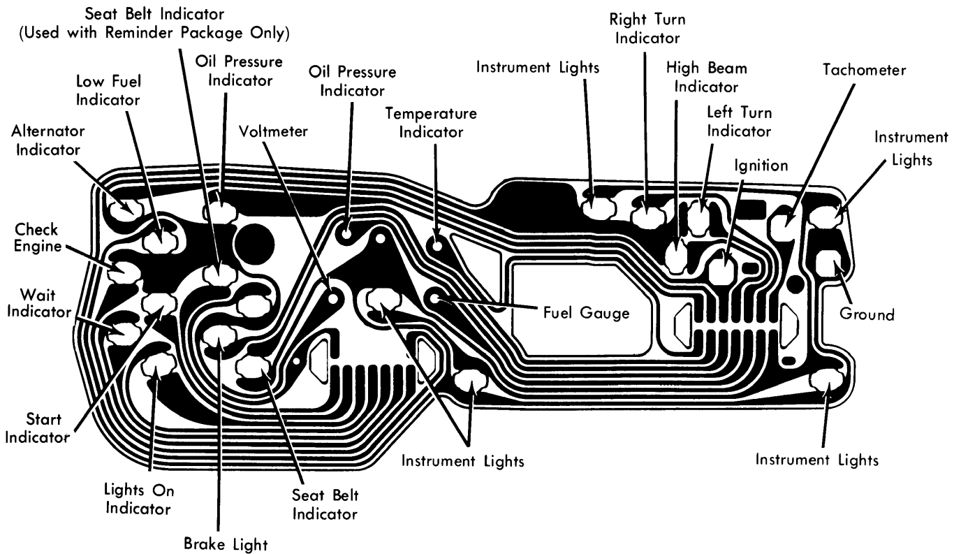
Cutlass Instrument Cluster with Gauges
