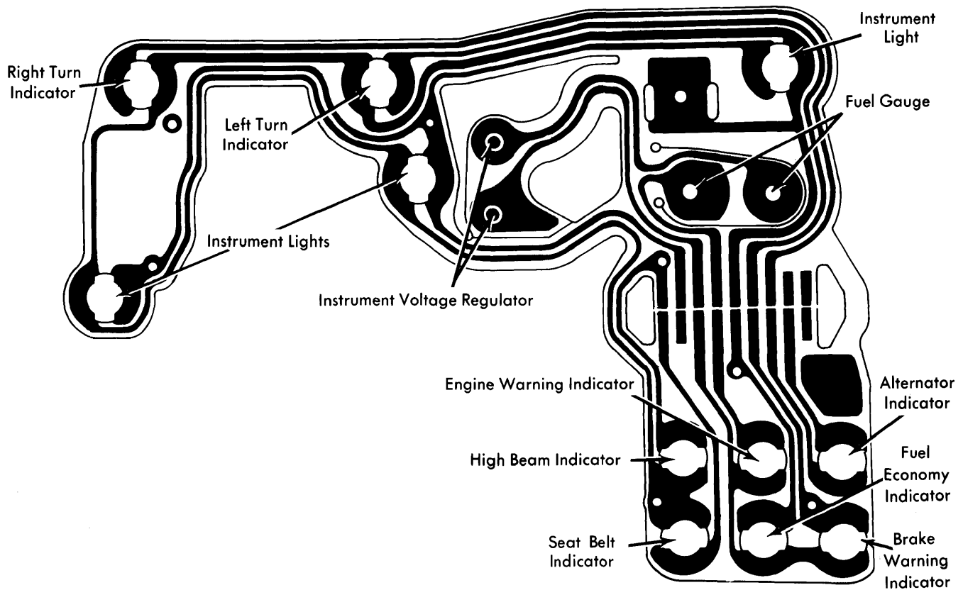
Lincoln Versailles Instrument Cluster
