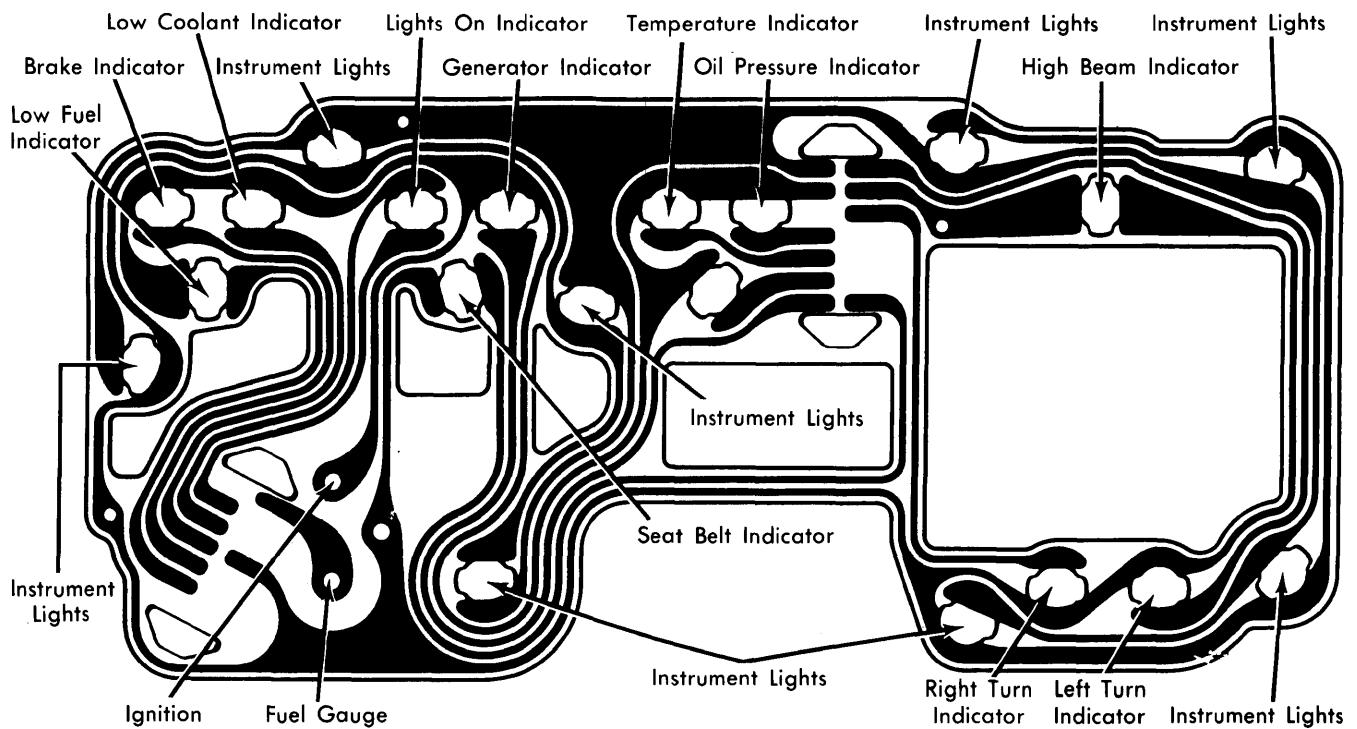
Omega Instrument Cluster with Indicator Lights
