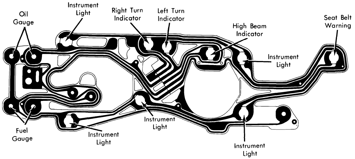
Capri, Mustang, Fairmont and Zephyr Primary Instrument Cluster with Tachometer
