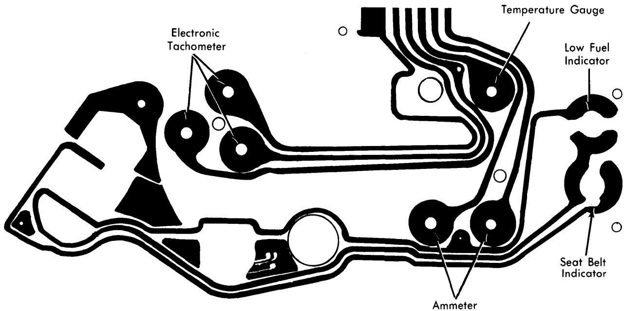
Capri, Mustang, Fairmont and Zephyr Secondary Instrument Cluster with Tachometer
