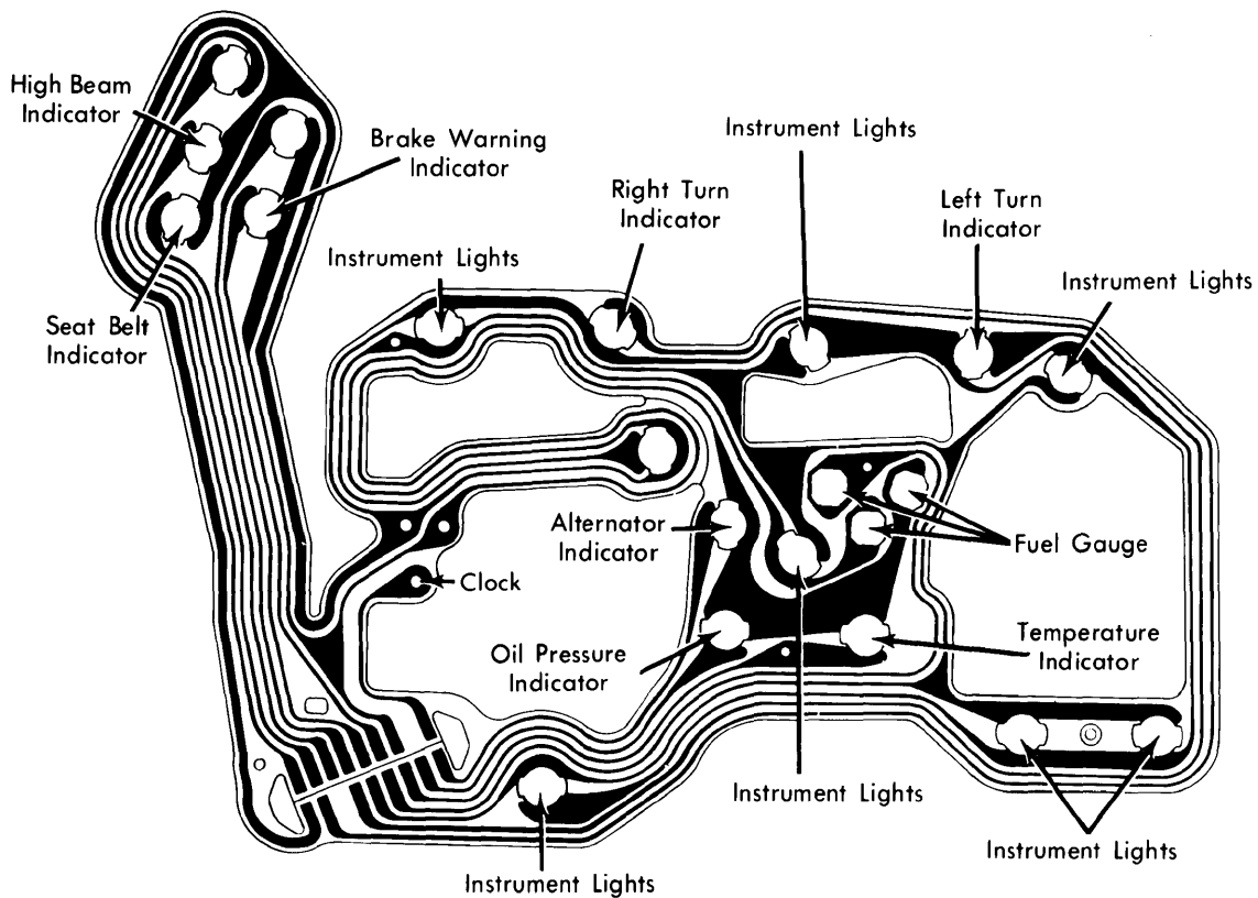
Caballero, El Camino, and Malibu Instrument Cluster without Gauges
