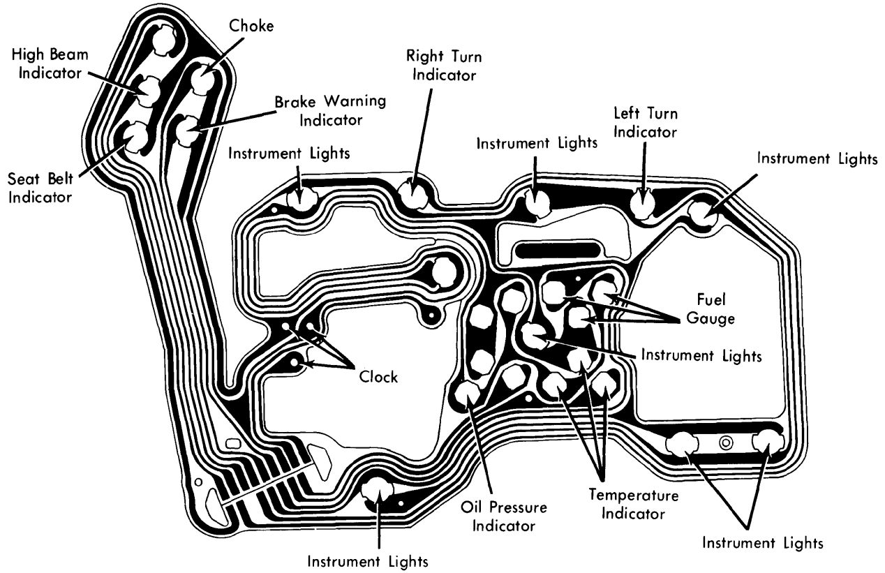
Caballero, El Camino, Malibu and Monte Carlo Instrument Cluster with Gauges
