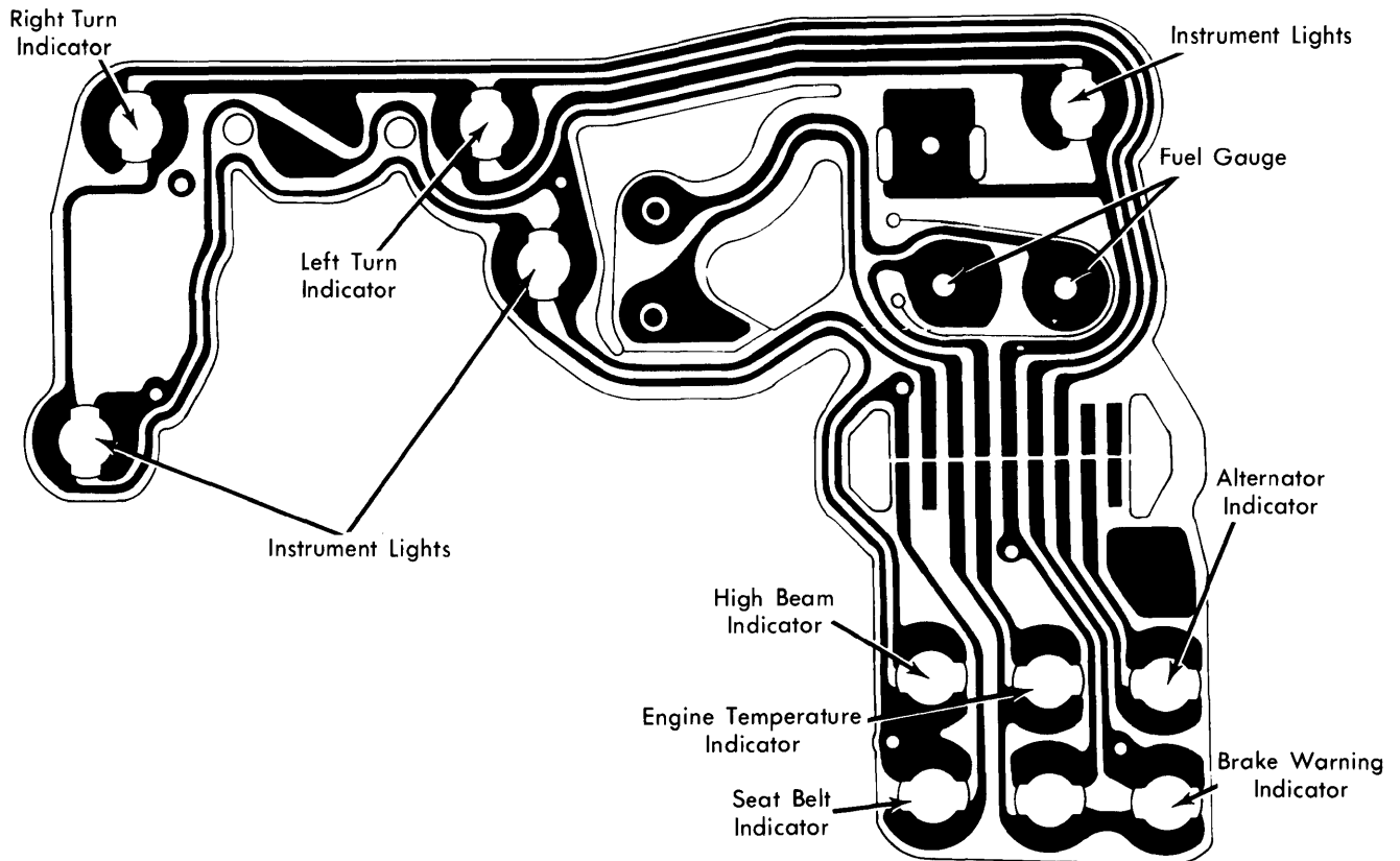
Granada and Monarch Instrument Cluster
