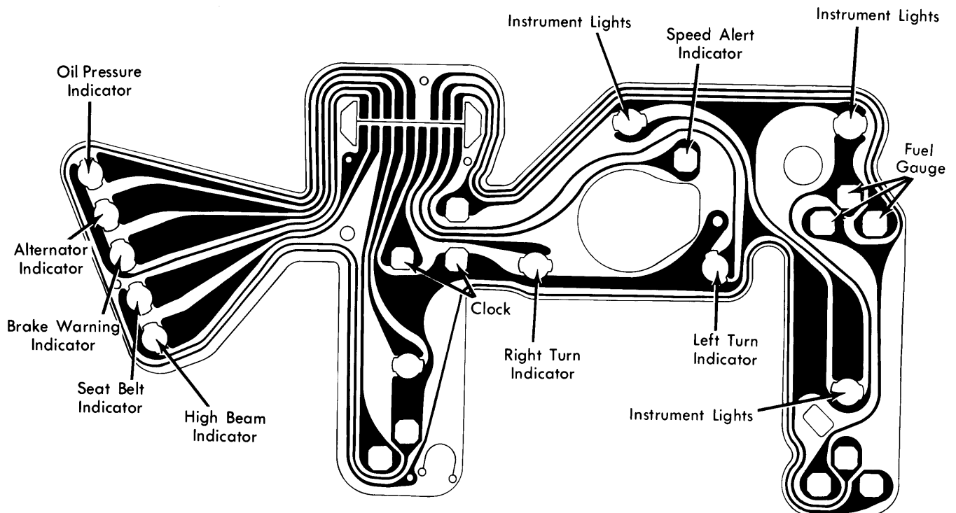
Century & Regal Instrument Cluster with Gauges
