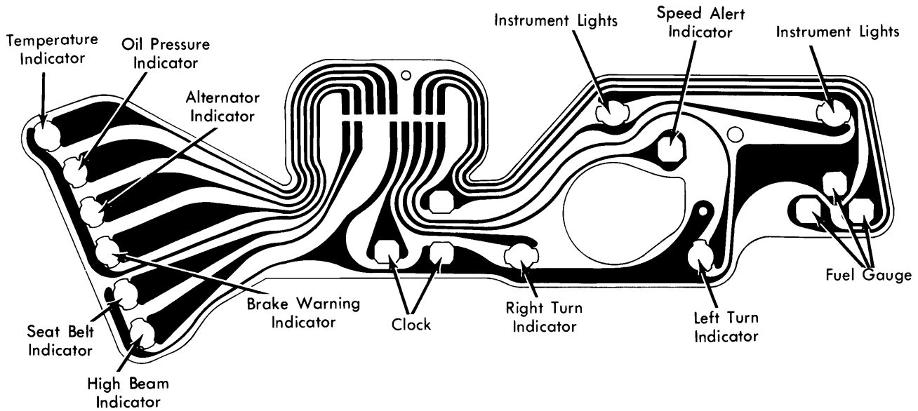
Century & Regal Instrument Cluster without Gauges
