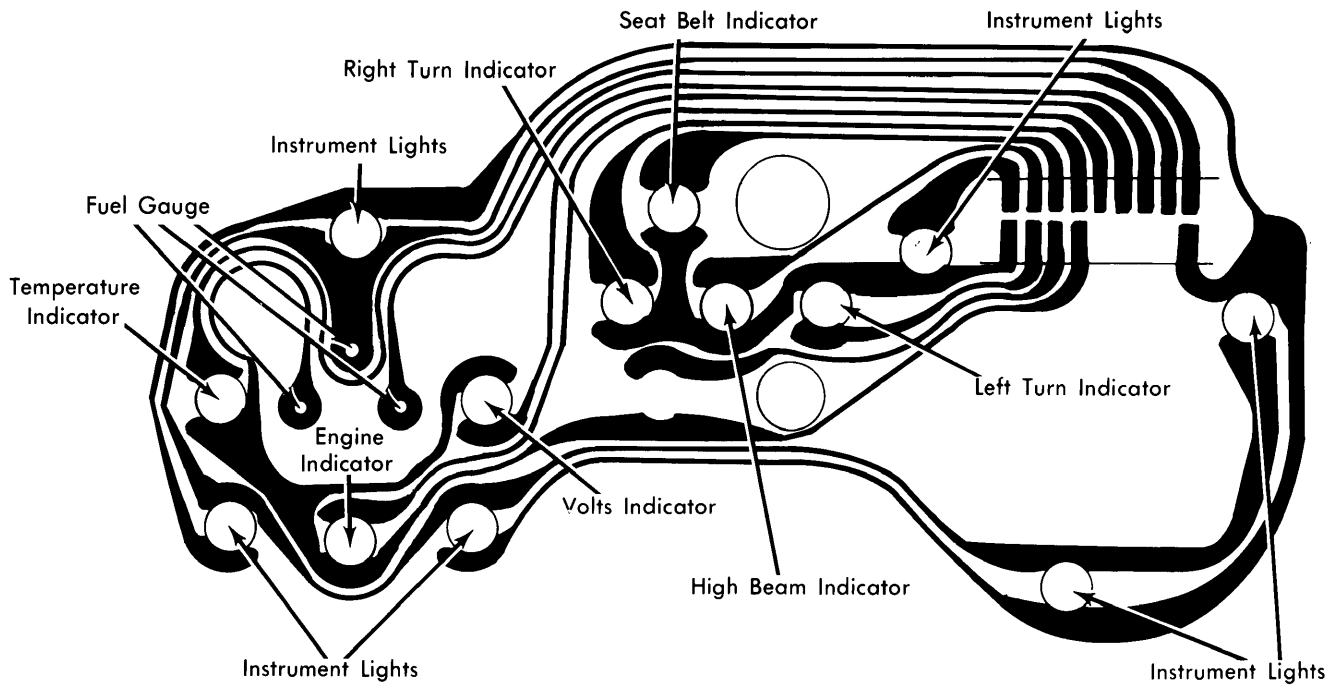
Skylark Instrument Cluster with Indicator Lights
