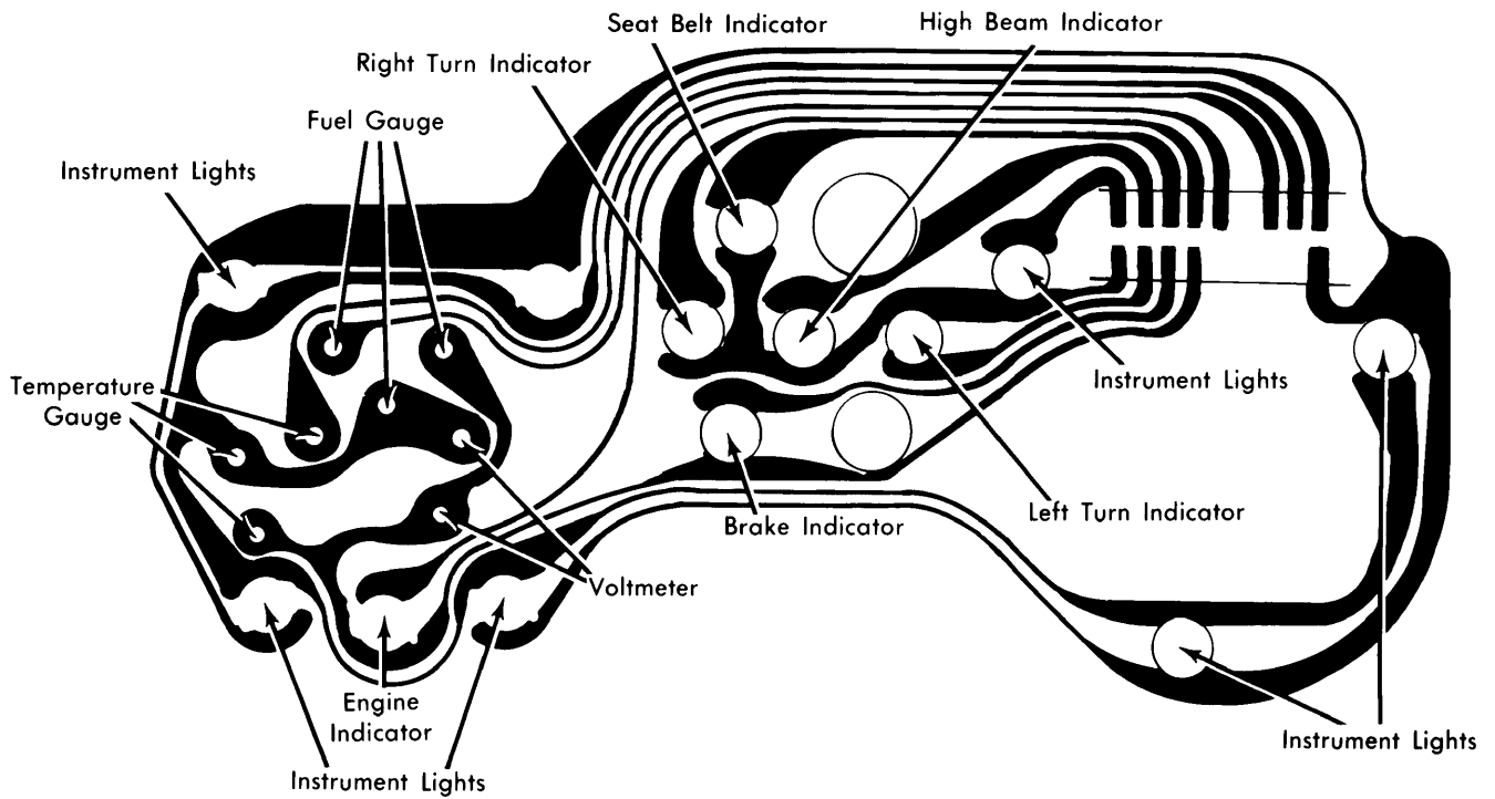
Skylark Instrument Cluster with Gauges
