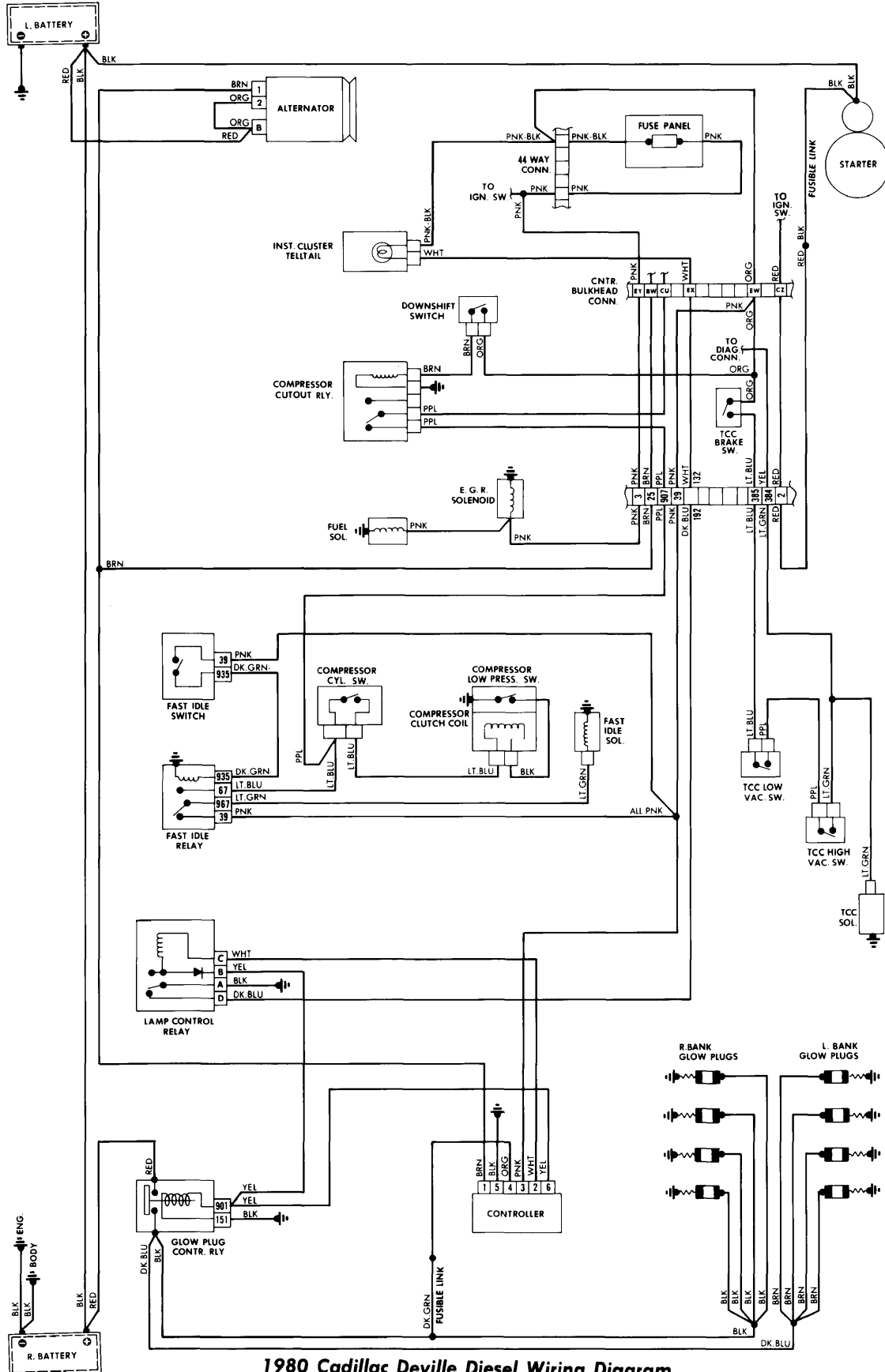
1980 Cadillac Deville Diesel Wiring Diagram For Complete Wiring, See Deville Gasoline Engine Wiring Diagram
