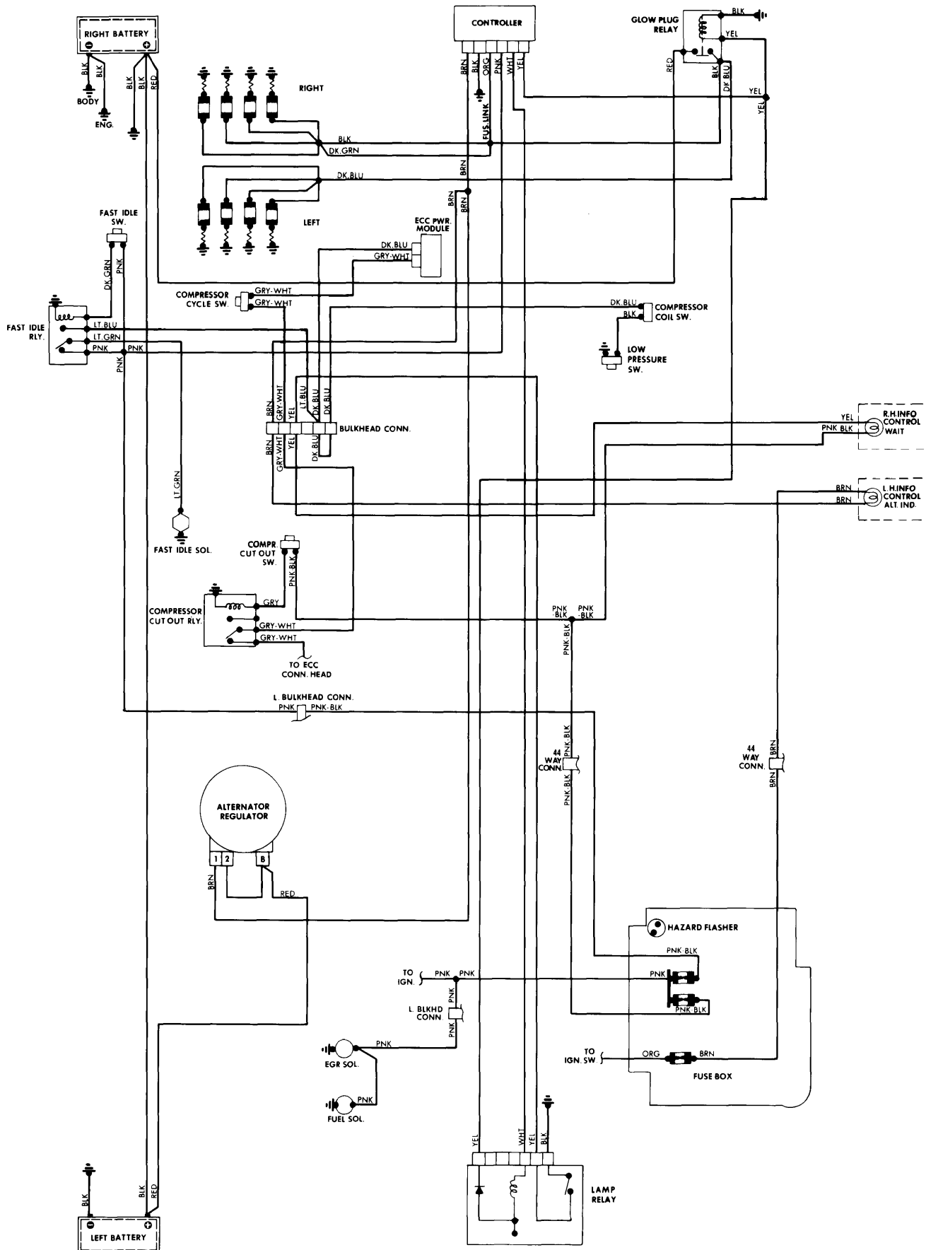
1980 Cadillac Eldorado & Seville Diesel Wiring Diagram. For Complete Wiring, See Cadillac Gasoline Engine Wiring Diagram
