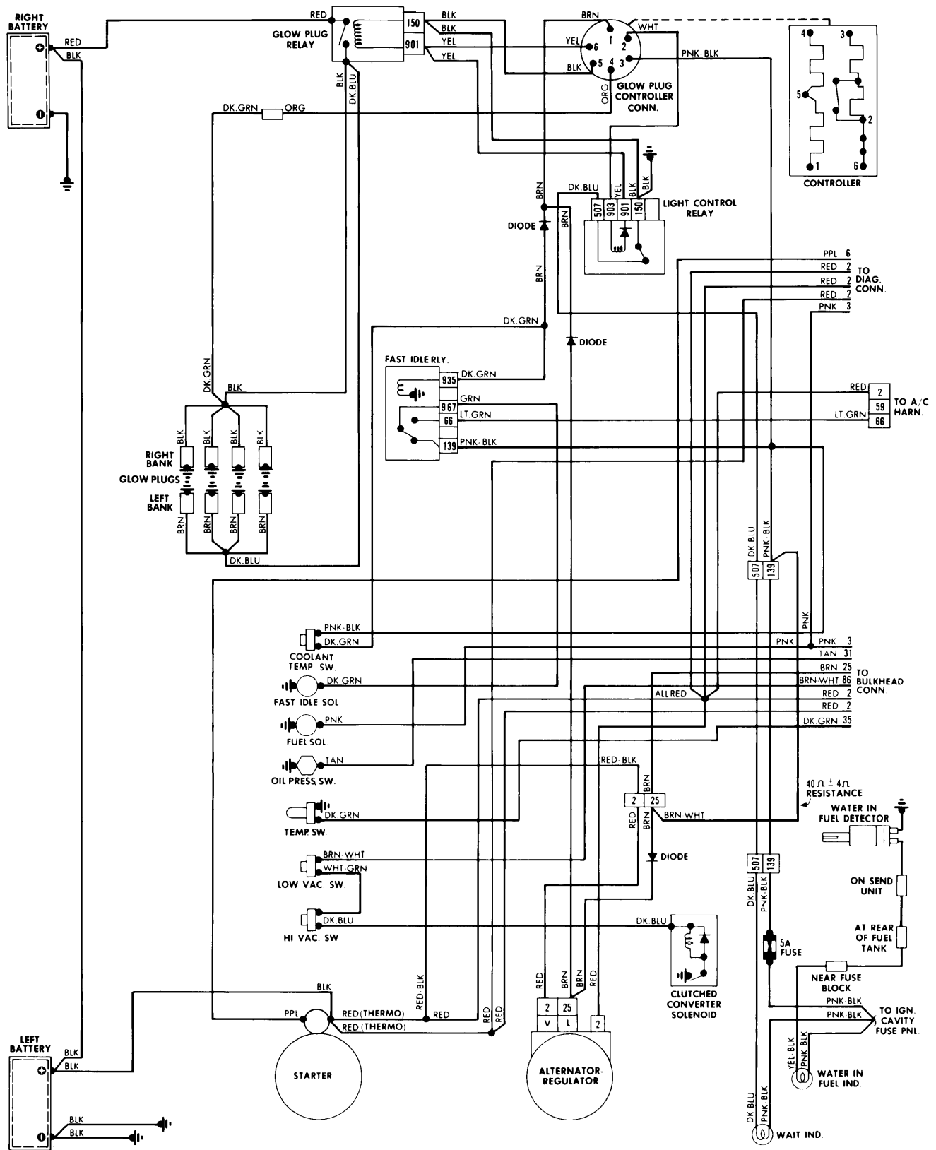
1980 General Motors (Exc. Cadillac & Cutlass) Diesel Engine Wiring Diagram. For Complete Wiring, See General Motors Gasoline Engine Wiring Diagrams
