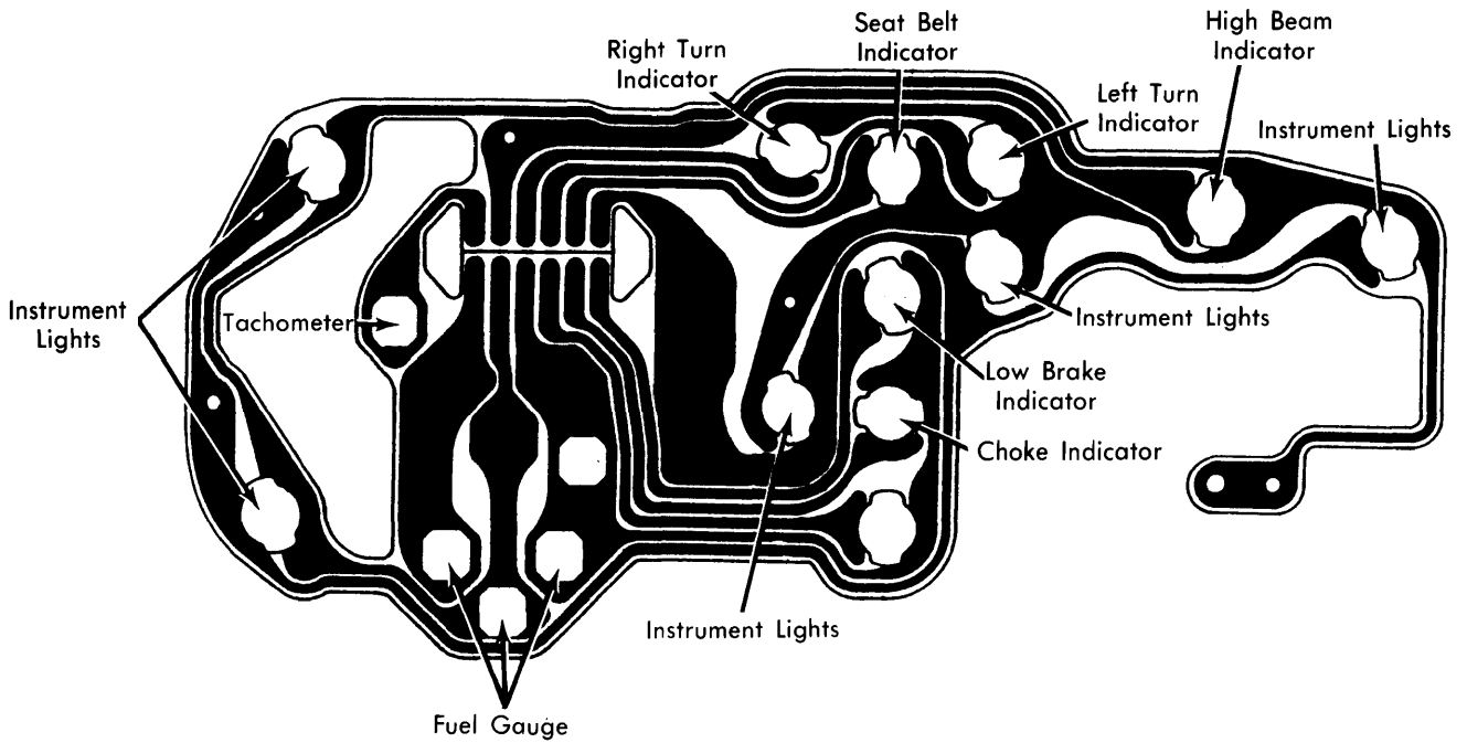
Phoenix Instrument Cluster with Tachometer
