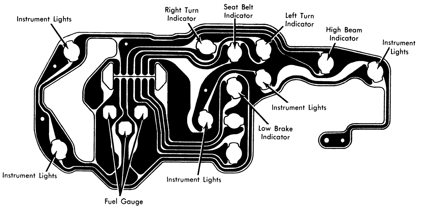
Phoenix Instrument Cluster without Tachometer
