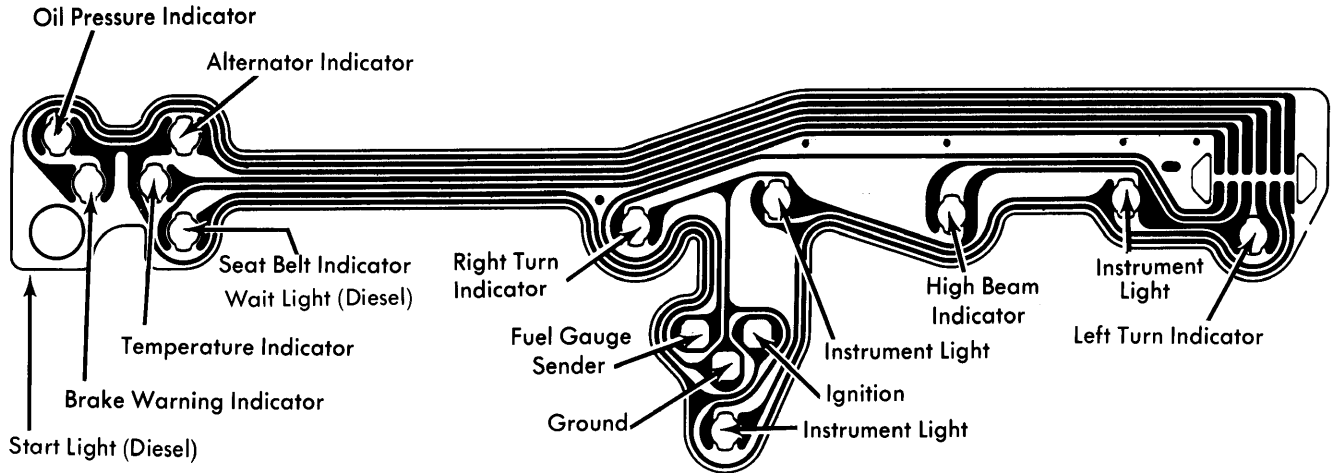
Delta 88 and Ninety Eight Instrument Cluster
