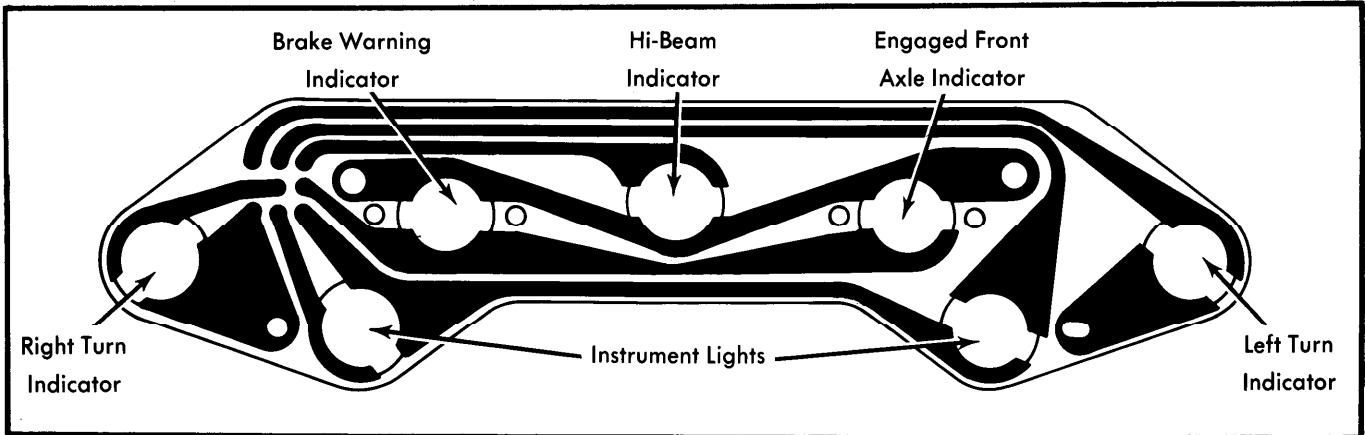
International Harvester Scout II, Terra and Traveler Speedometer Circuit
