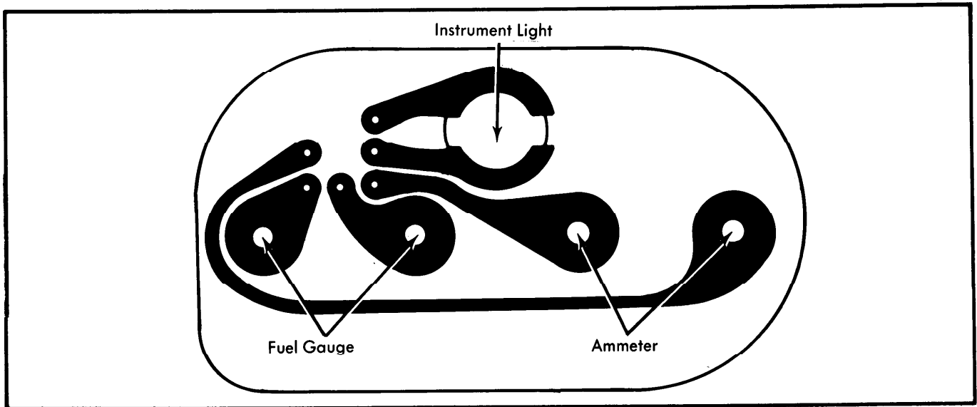
International Harvester Scout II, Terra and Traveler Ammeter and Fuel Gauge Circuit
