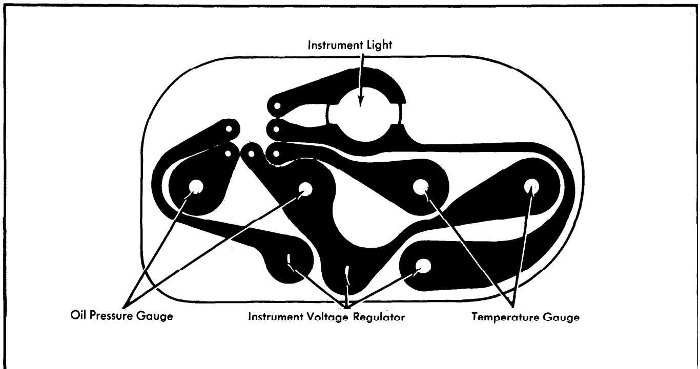
International Harvester Scout II, Terra and Traveler Temperature and Oil Pressure Gauge Circuit
