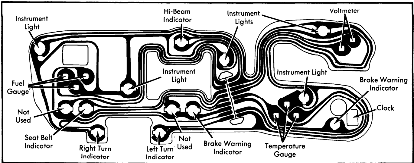
Chevrolet and GMC "C" and "K" (All Models) With Clock and Gauges, No Tachometer
