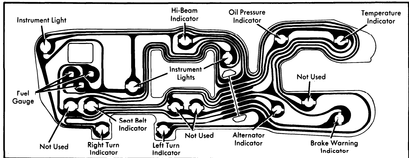
Chevrolet and GMC "C" and "K" (All Models) Without Tachometer and Clock, No Gauges
