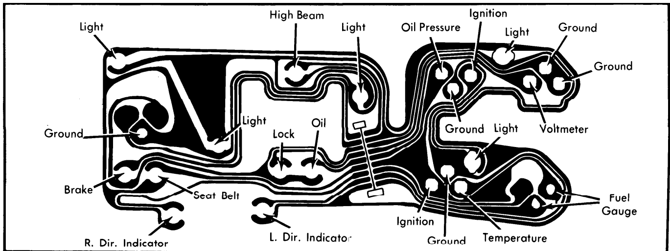
Chevrolet and GMC "C" and "K" (All Models) With Tachometer and Gauges, No Clock
