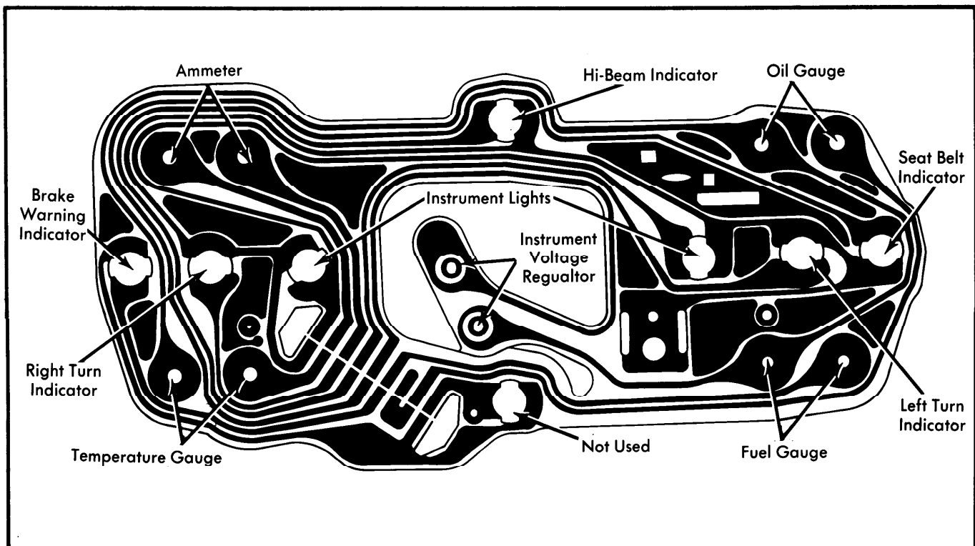
Ford Motor Co. All Models With Ammeter and Oil Pressure Gauge
