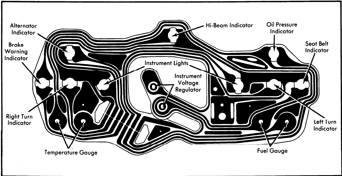
Ford Motor Co. All Models With Alternator and Oil Pressure Indicator Lights
