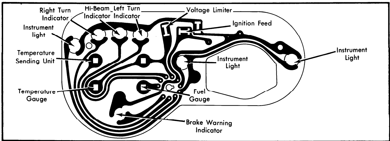
Chrysler Corp. "B", "CB", "MB" and "PB" Models
