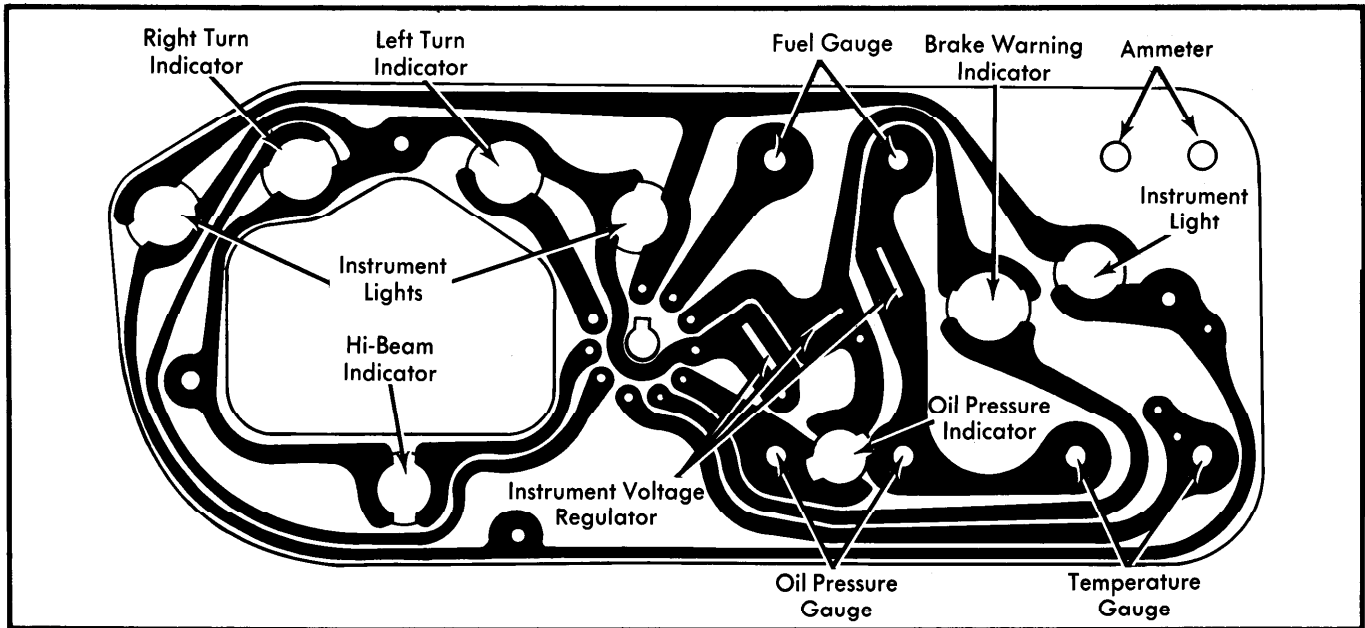
Chrysler Corp. "AD", "AW", "D", "PD", "PW" and "W" Models
