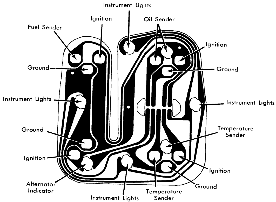
LeMans & Grand Prix Auxiliary Instrument Cluster
