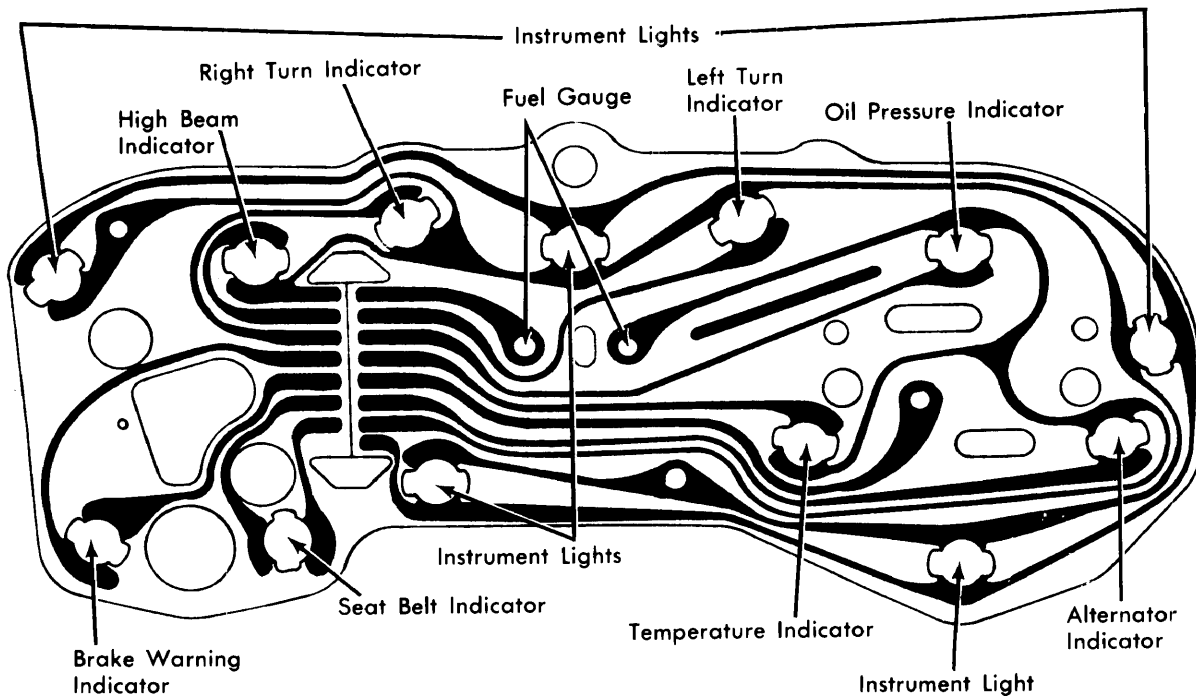
Firebird Instrument Cluster with Indicator Lights
