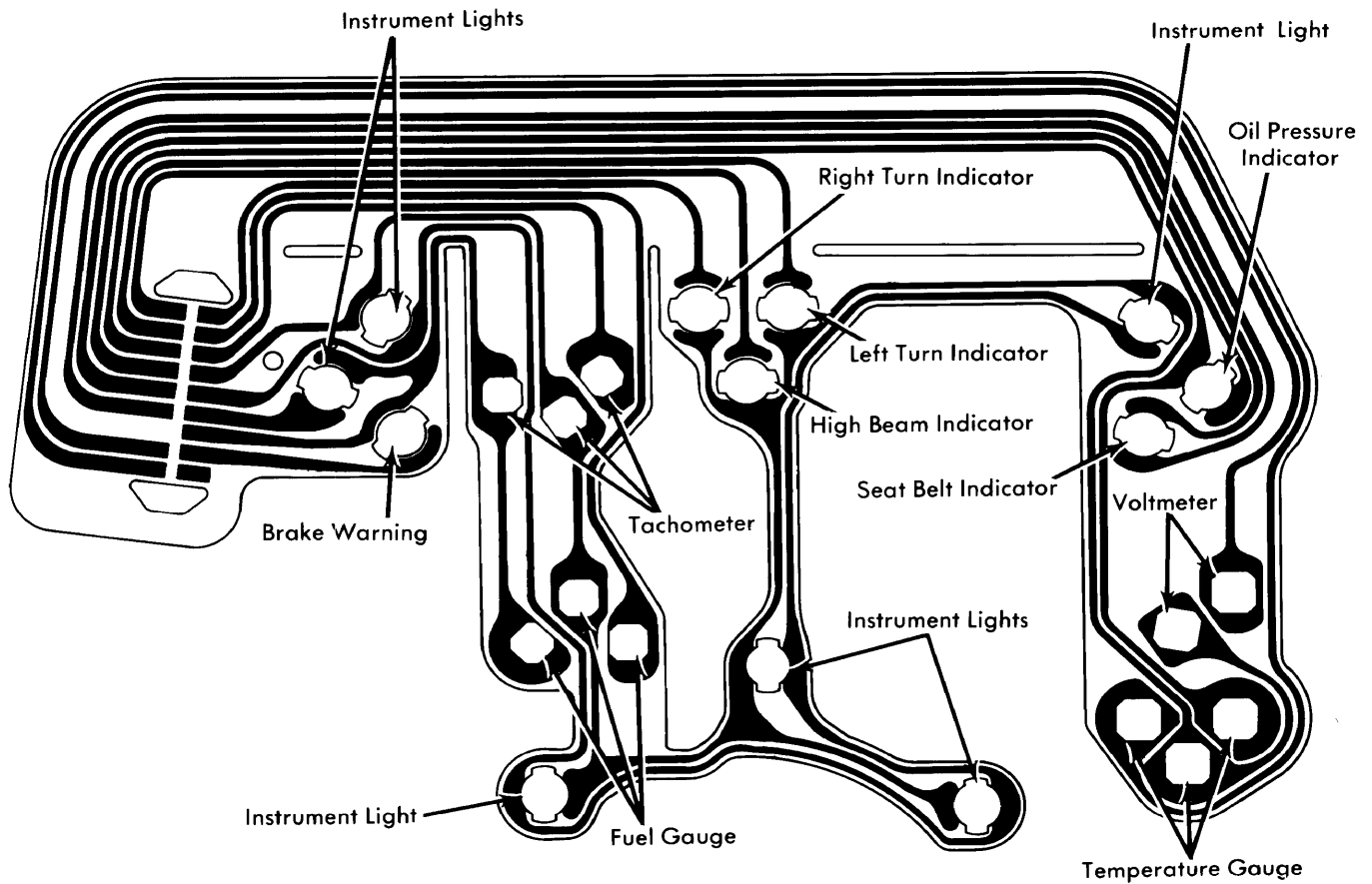
Sunbird Instrument Cluster with Gauges
