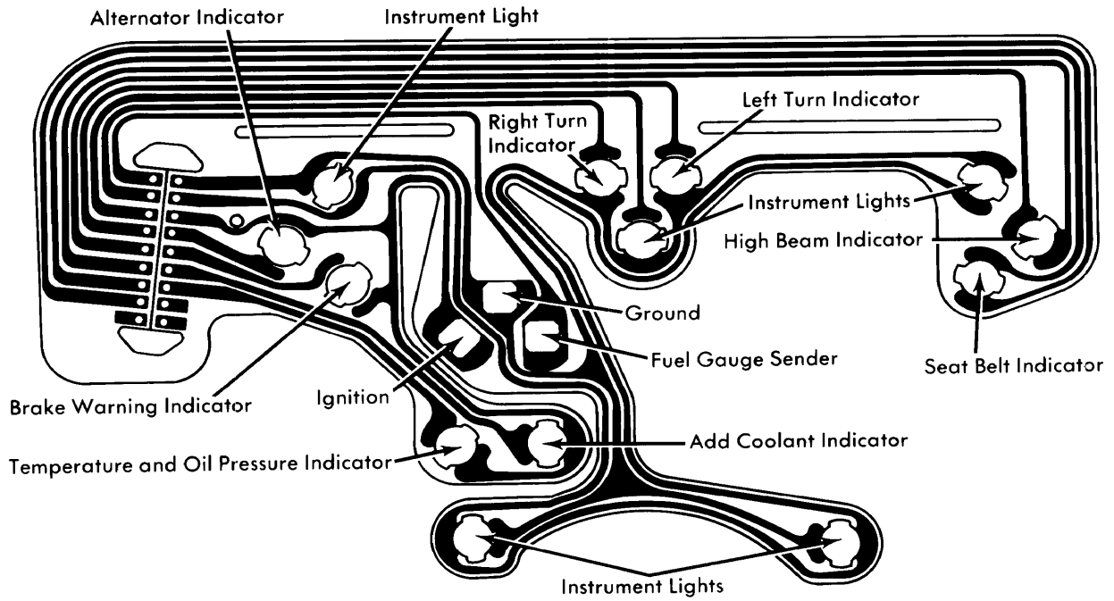
Sunbird Instrument Cluster with Indicator Lights
