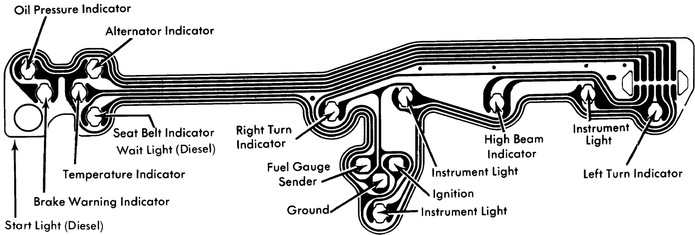
Delta 88 and Ninety Eight Instrument Cluster
