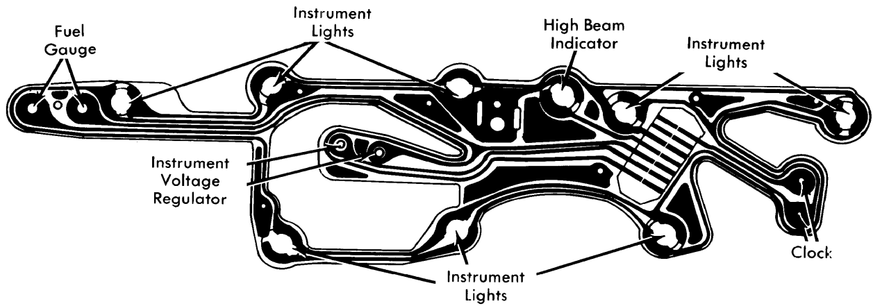
Lincoln Continental Mark V Instrument Cluster
