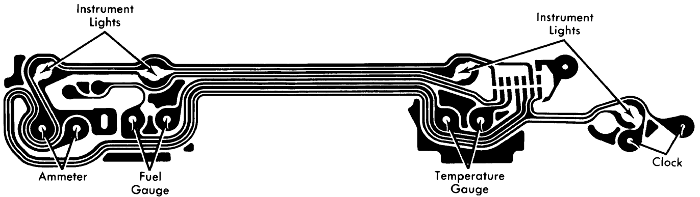
Lincoln Continental Lower Instrument Cluster
