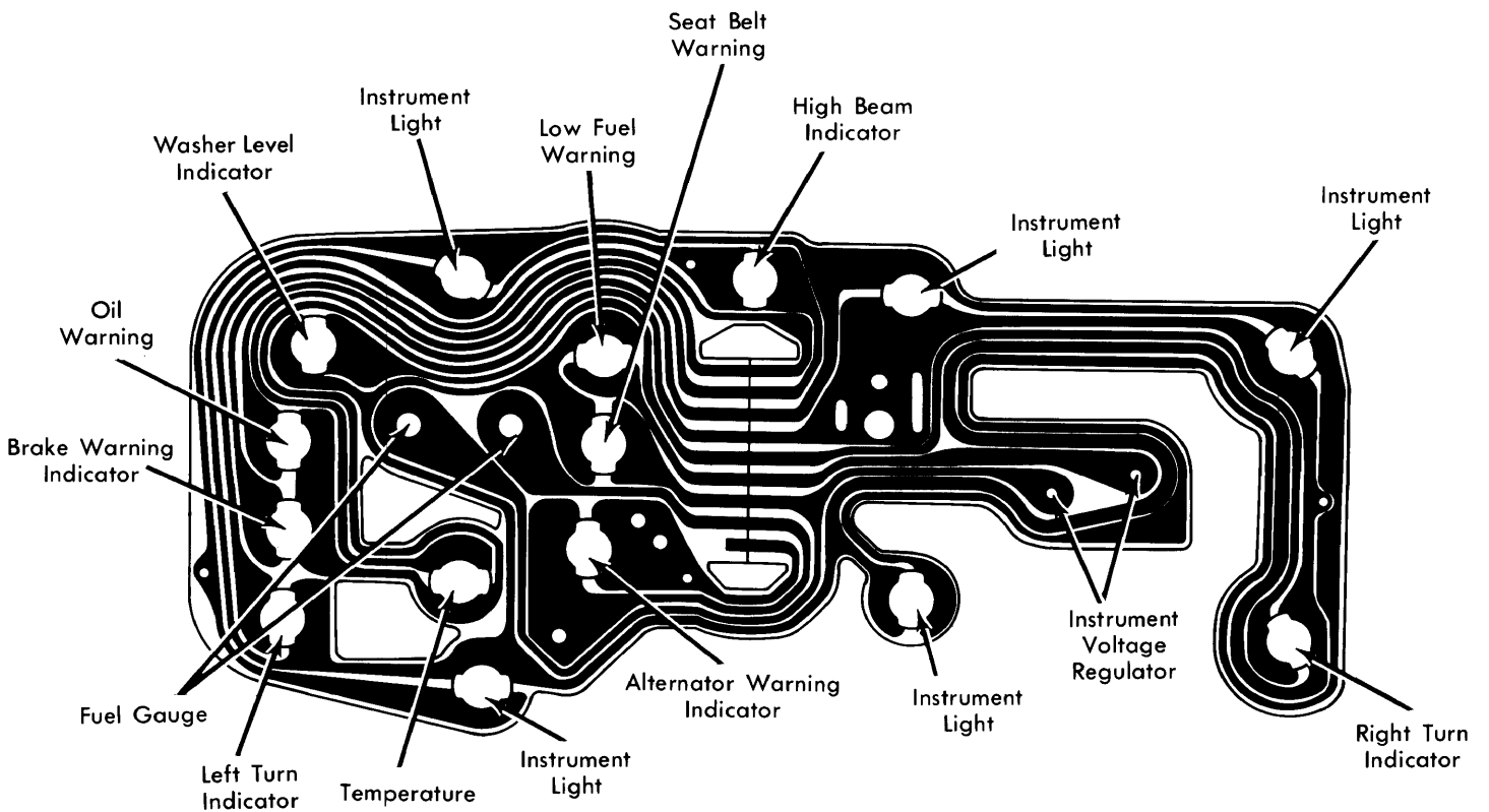
Mercury Instrument Panel
