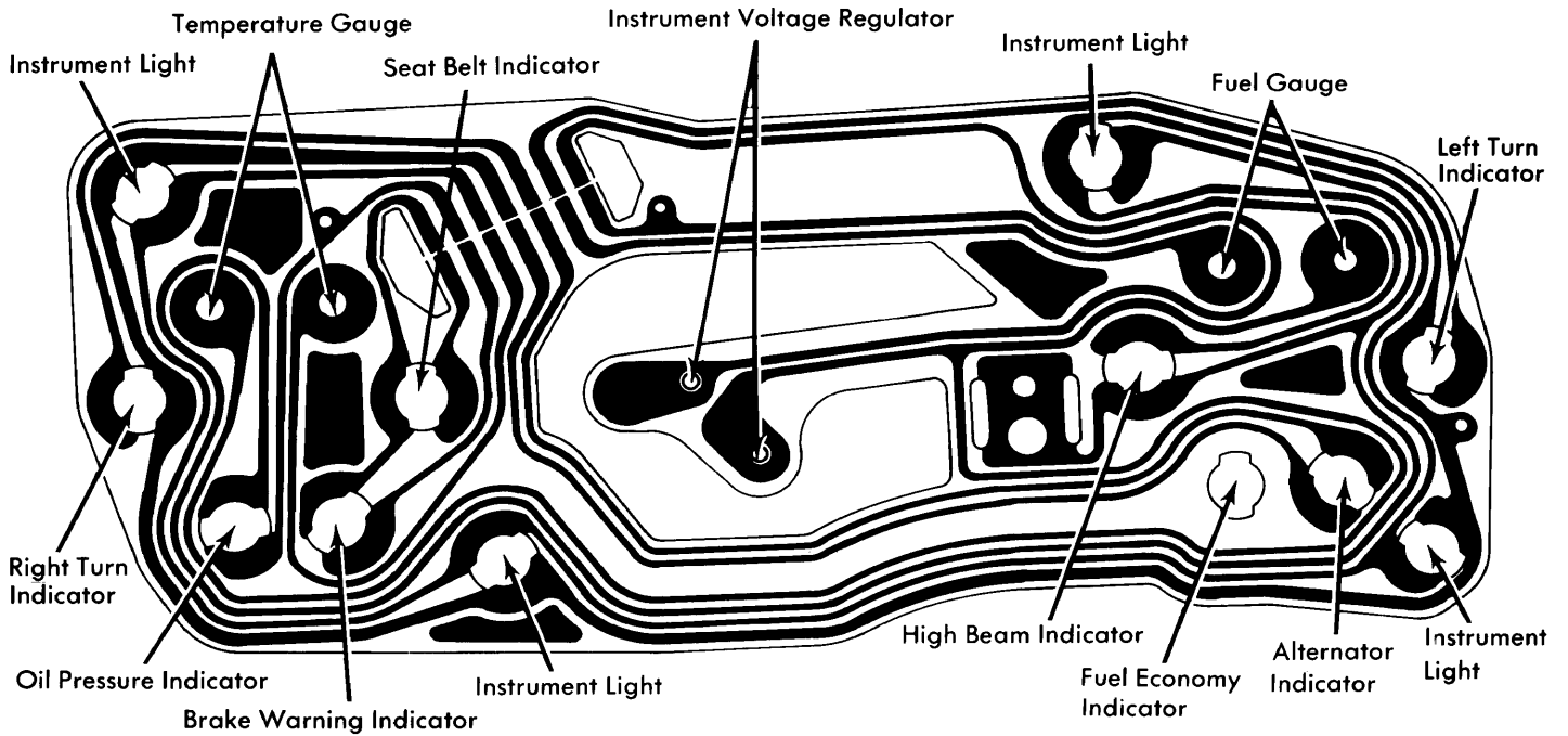
LTD II, Thunderbird, and Cougar Instrument Cluster
