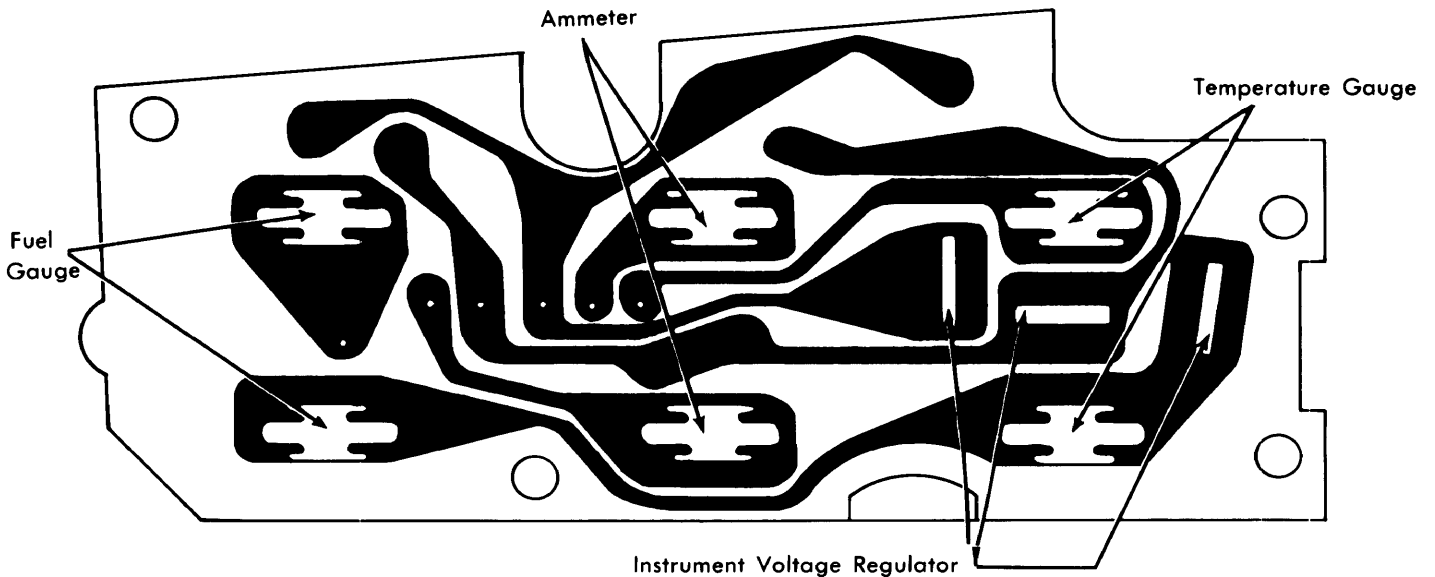
Chrysler and St. Regis Instrument Gauge Cluster
