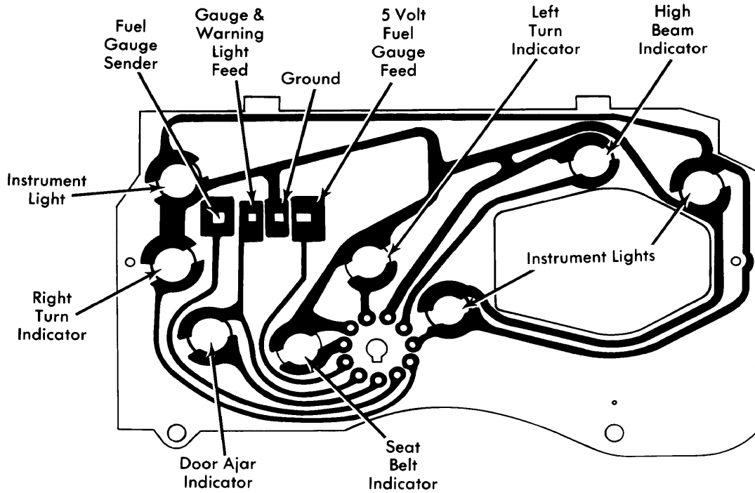
Diplomat and LeBaron Instrument Cluster with Gauges
