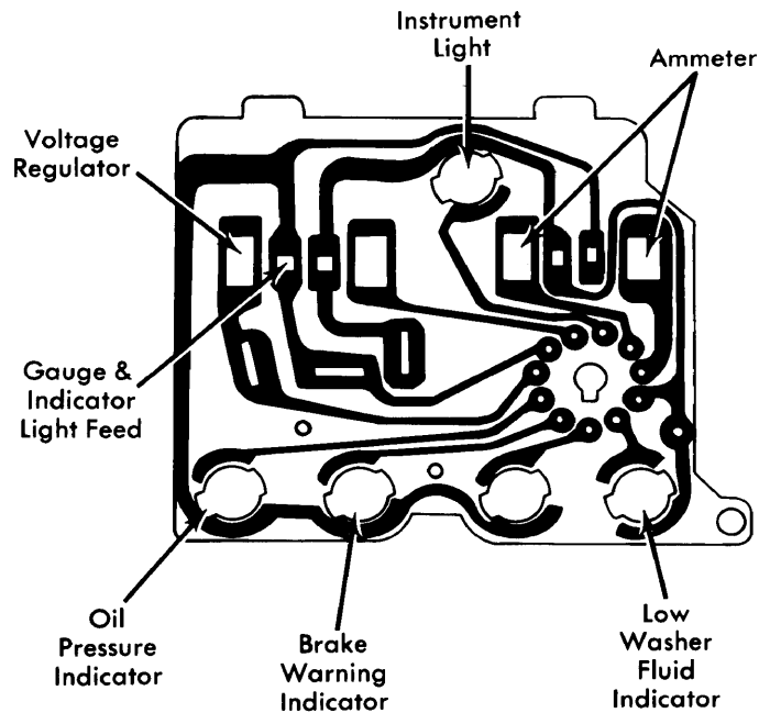
Diplomat and LeBaron Instrument Cluster without Gauges
