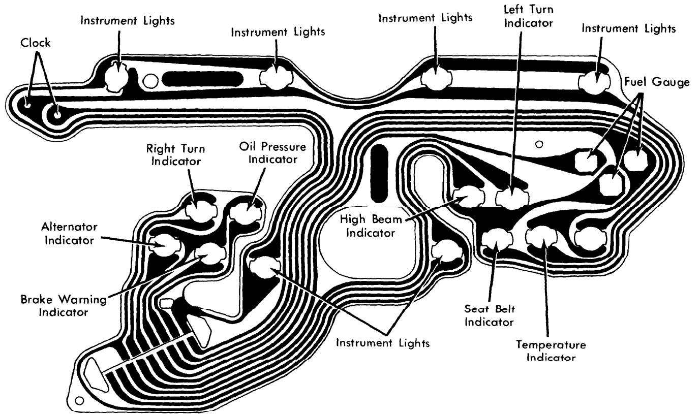
Monte Carlo Instrument Cluster without Gauges
