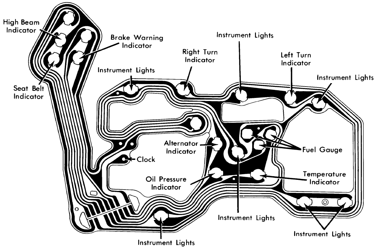
Malibu, Monte Carlo, El Camino and Caballero Instrument Cluster without Gauges
