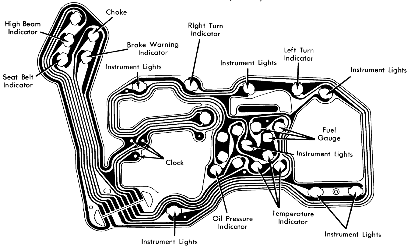
Malibu, Monte Carlo, El Camino and Caballero Instrument Cluster with Gauges
