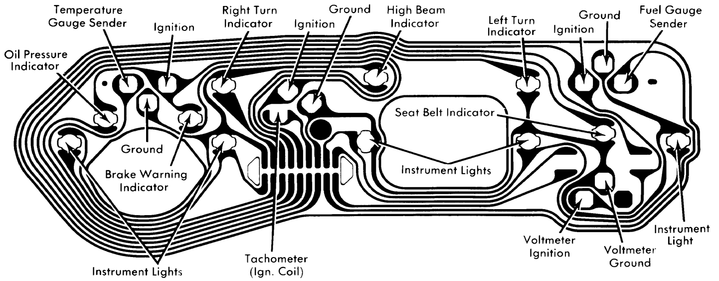
Nova Instrument Cluster with Gauges
