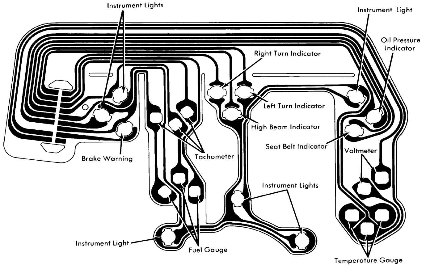
Monza Instrument Cluster with Gauges
