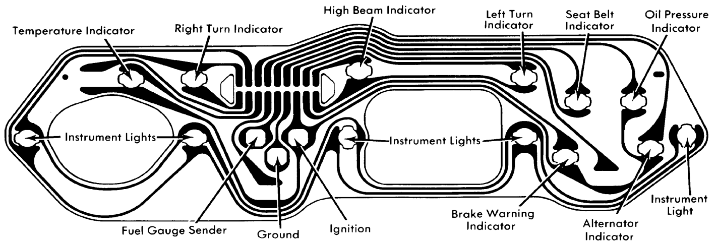
Nova Instrument Cluster with Indicator Lights
