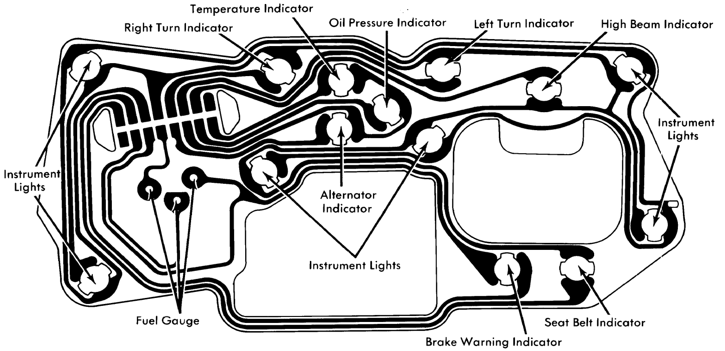
Chevette Instrument Cluster with Indicator Lights
