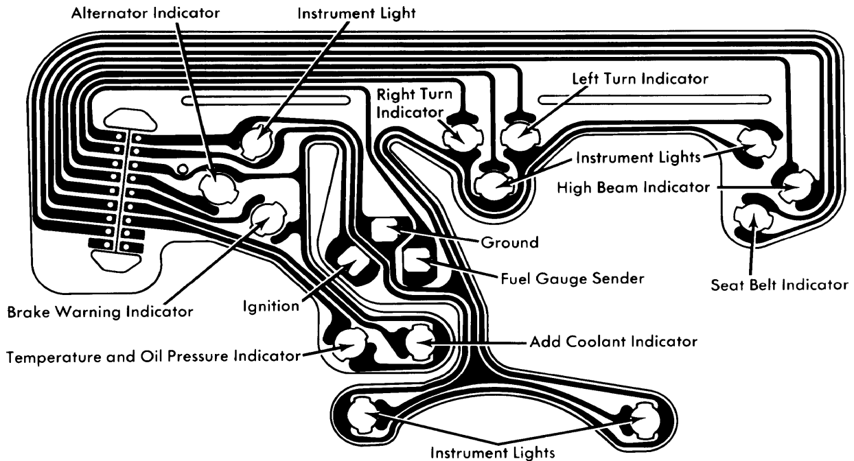
Monza Instrument Cluster with Indicator Lights
