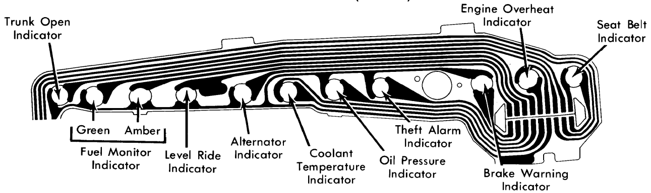
Seville Instrument Cluster with Digital Readout
