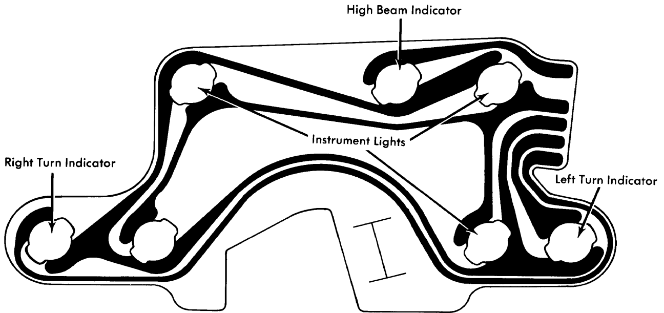
Cadillac (except Seville and Eldorado) Speedometer Cluster
