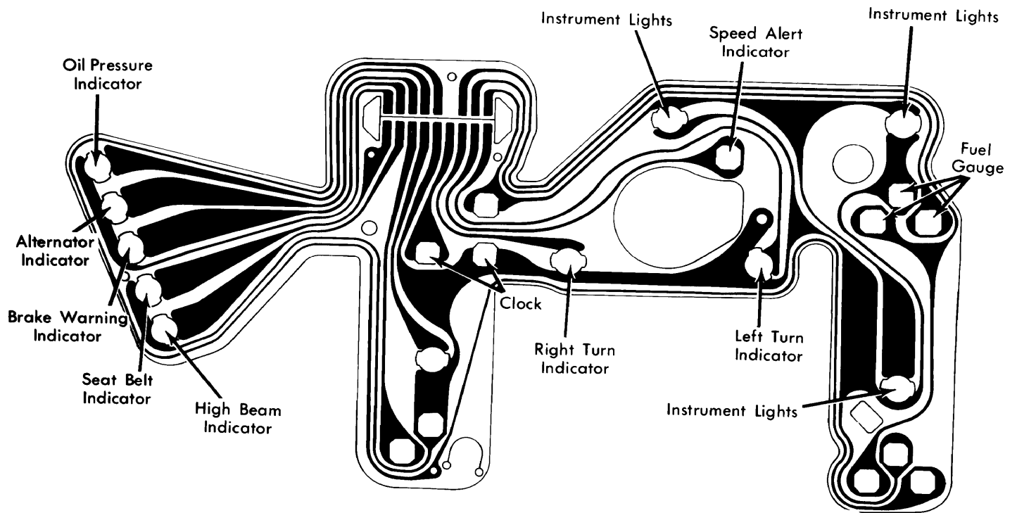
Century & Regal Instrument Cluster with Gauges
