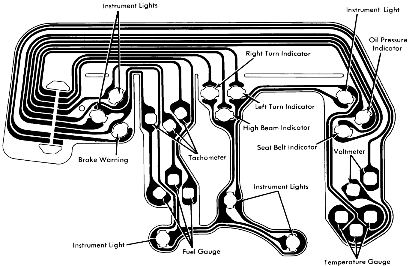
Skyhawk Instrument Cluster with Gauges
