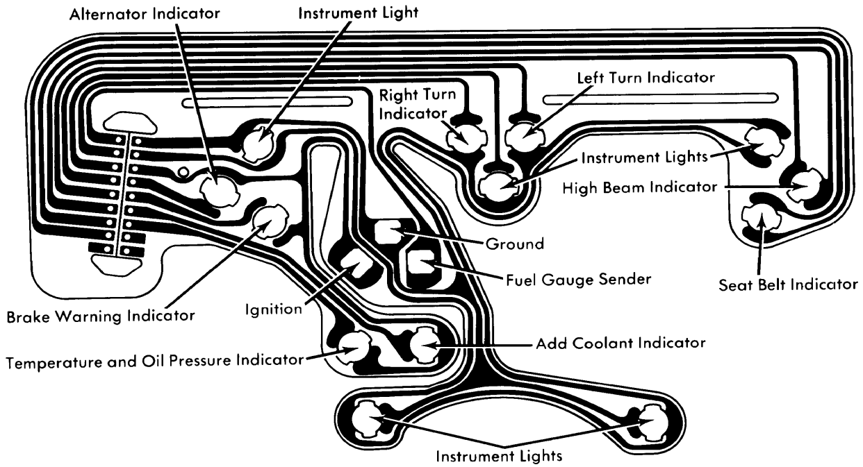
Skyhawk Instrument Cluster with Indicator Lights
