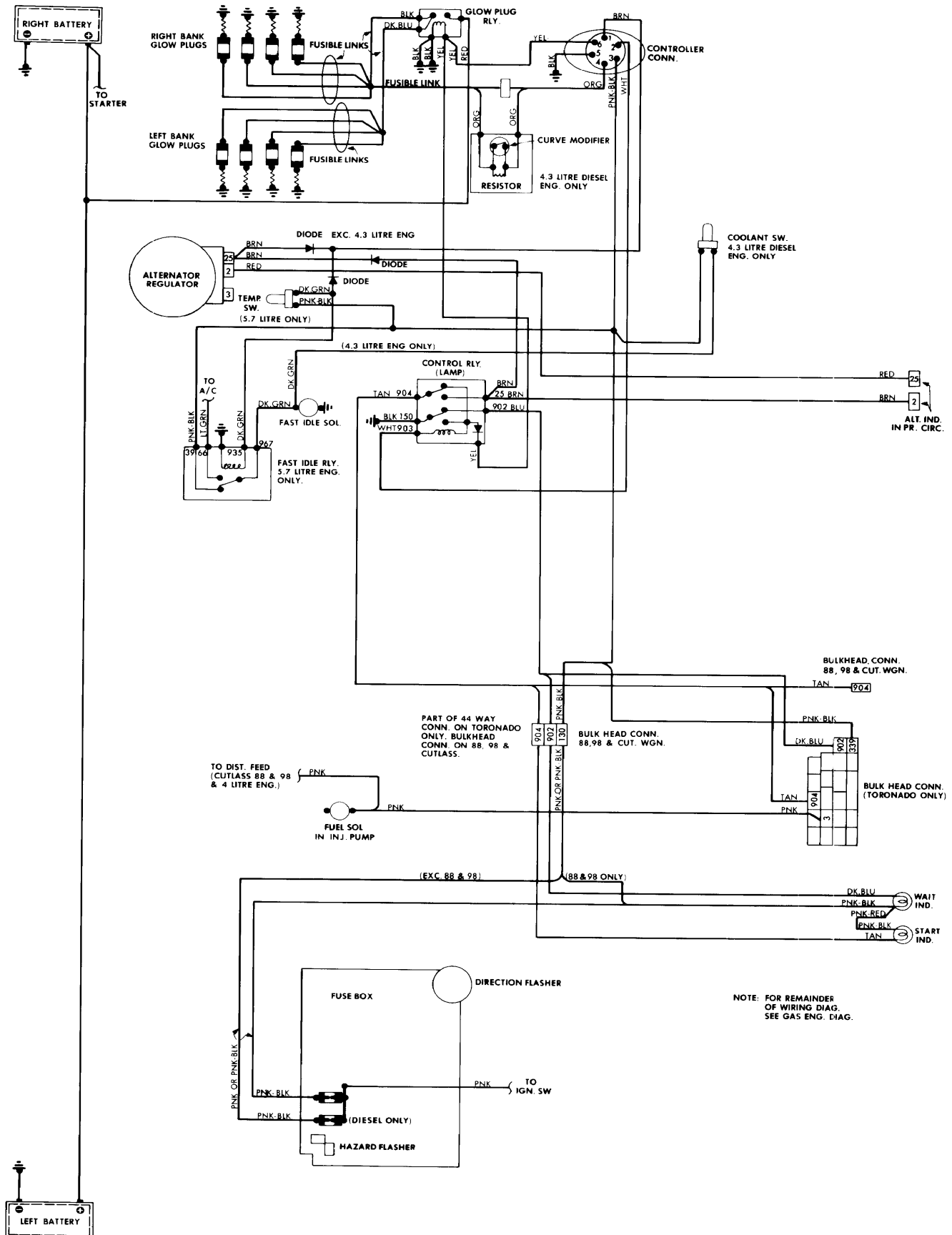
1979 Oldsmobile Type 2 Diesel Wiring Diagram
