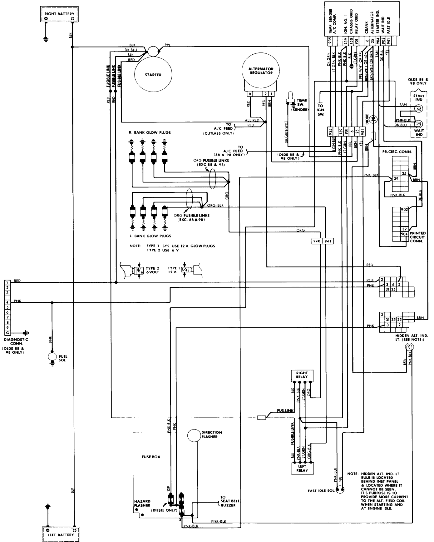
1979 Oldsmobile Type 1 Diesel Wiring Diagram
