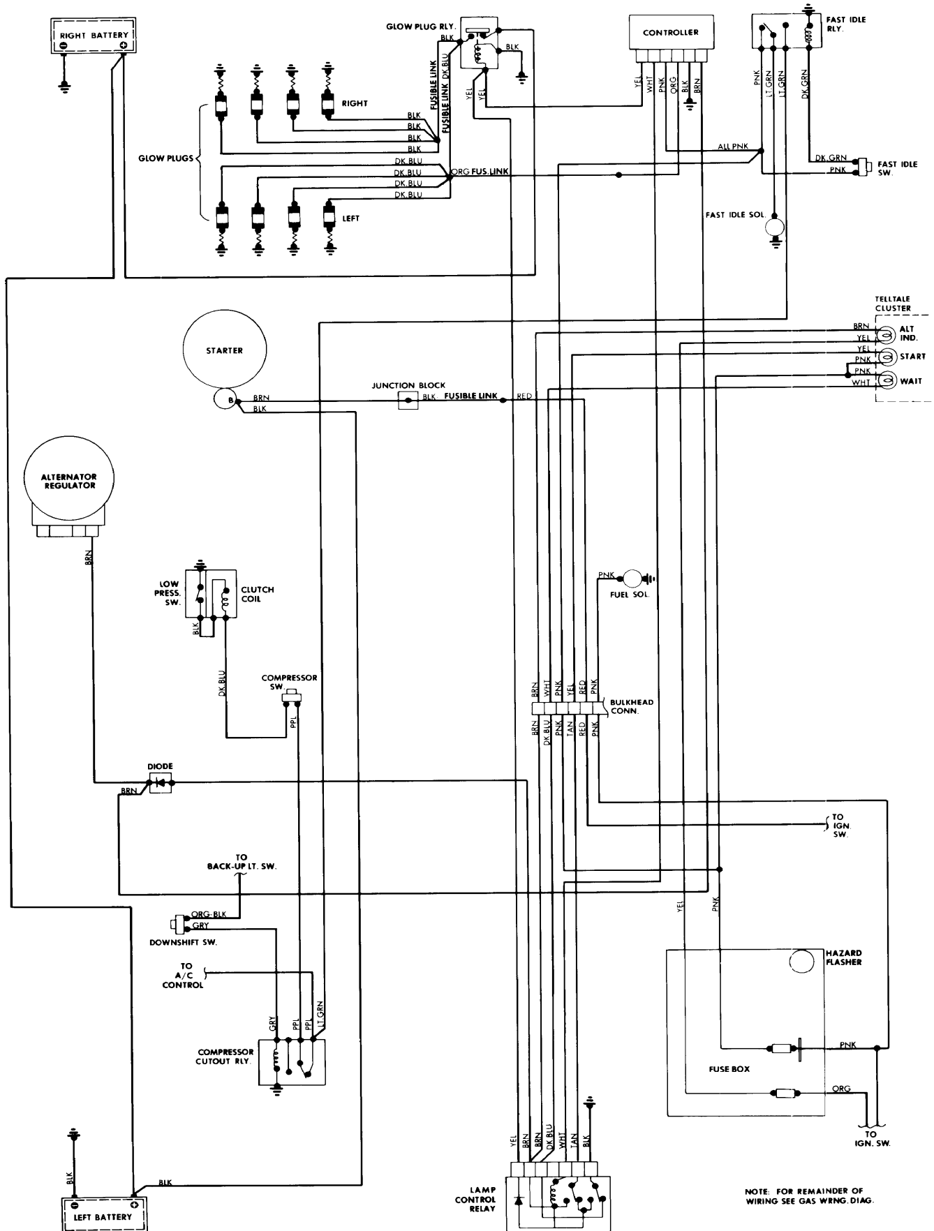
1979 Cadillac Seville Diesel Wiring Diagram
