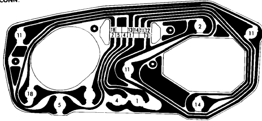
MAIN PRINTED CIRCUIT (W/GAUGE ONLY)
