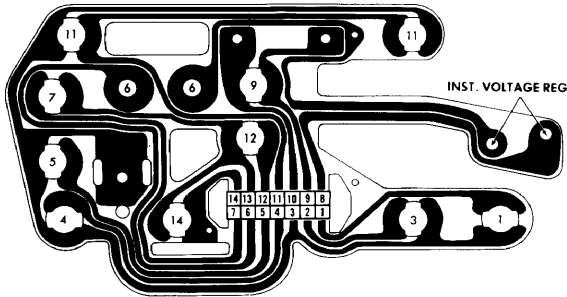
PRINTED CIRCUIT W/O GAUGE
