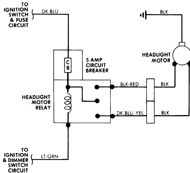
Chrysler Corp. Automatic Headlight Doors Wiring Diagram
