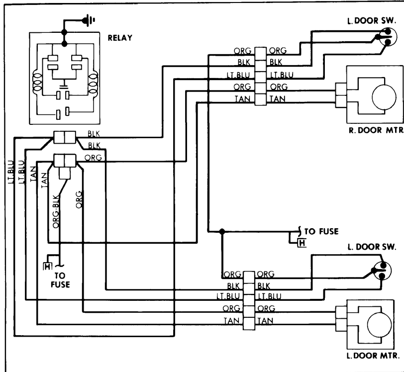
Buick Electra and Riviera Automatic Locking Electric Door Lock Wiring Diagram
