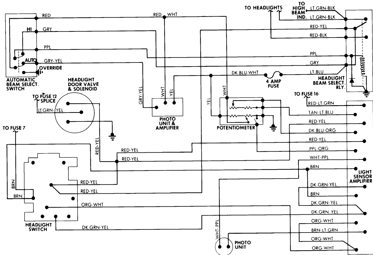
Lincoln Continental Automatic Headlights Autolamp Wiring Diagram
