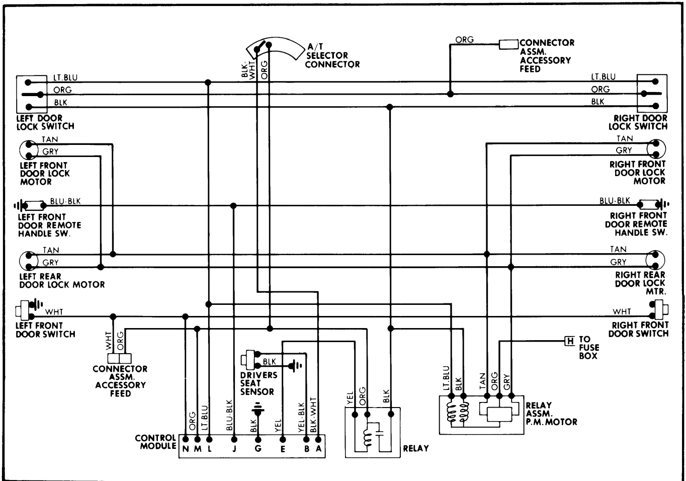
Cadillac Automatic Locking Electric Door Lock Wiring Diagram
