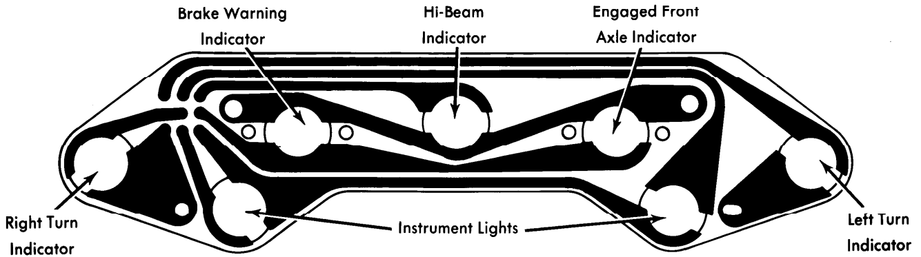
International Harvester Scout II, Terra and Traveler Speedometer Circuit
