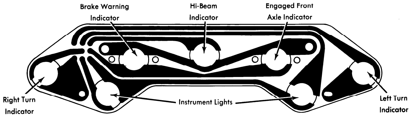
International Harvester Scout II, Terra and Traveler Speedometer Circuit
