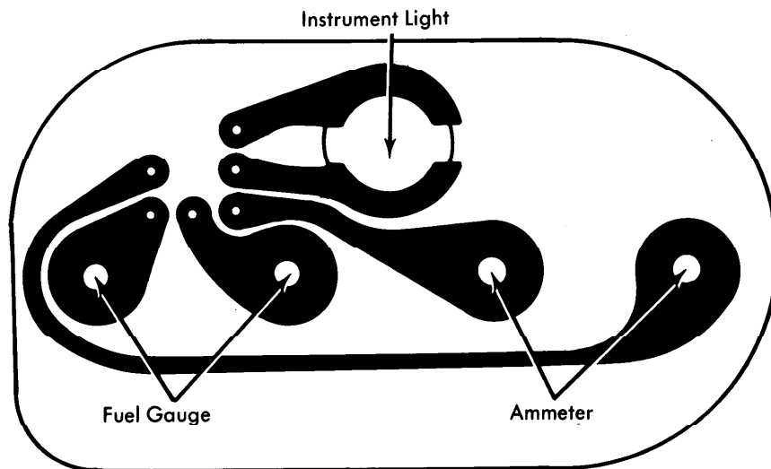
International Harvester Scout II, Terra and Traveler Ammeter and Fuel Gauge Circuit
