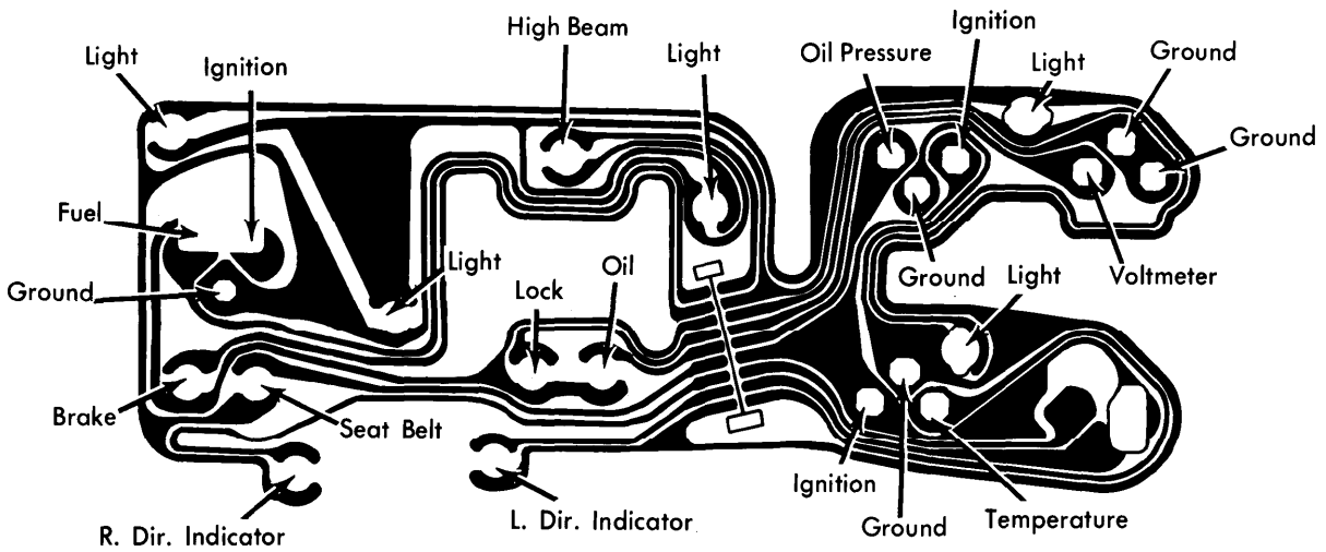
Chevrolet and GMC "C" and "K" (All Models) With Tachometer and Gauges, No Clock
