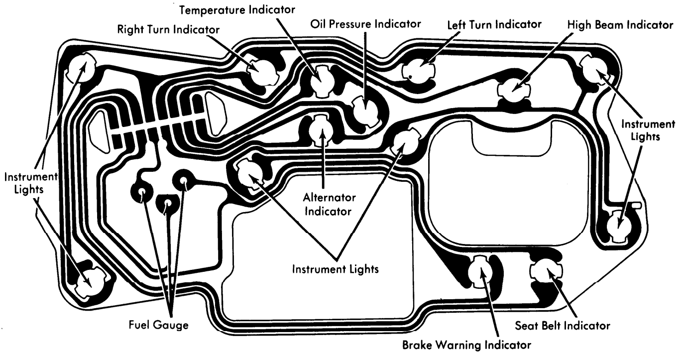
General Motors "G" Models (Without Gauges)
