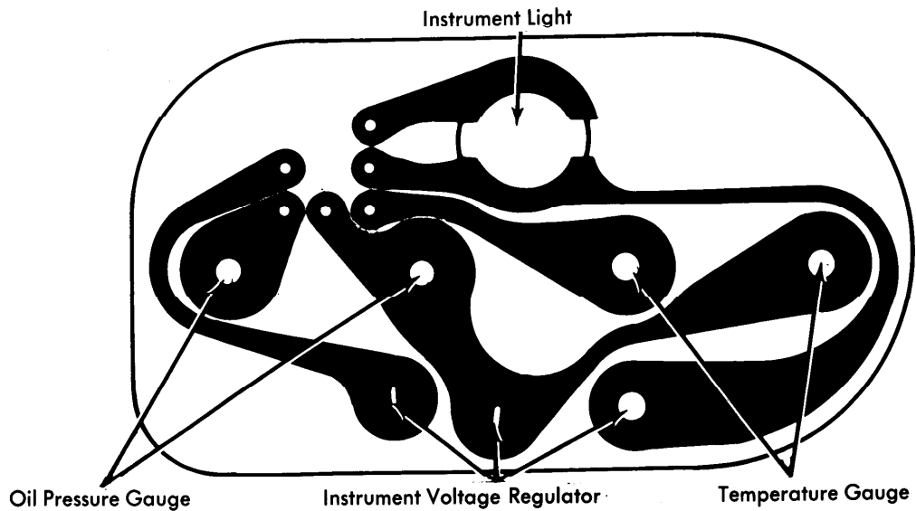
International Harvester Scout II, Terra and Traveler Temperature and Oil Pressure Gauge Circuit
