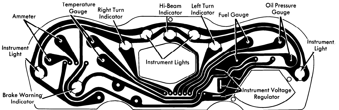
Chrysler Corp. (Motor Home Chassis) Models
