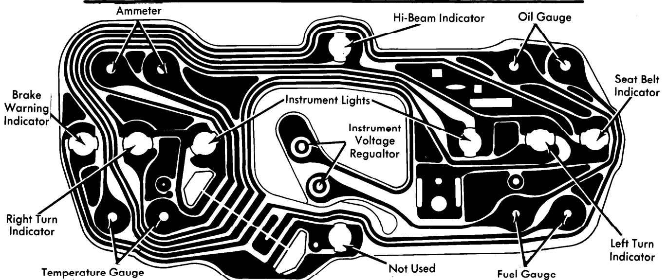
Ford "E" and "F" (All Models) With Ammeter and Oil Gauge
