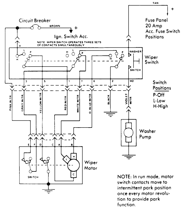
American Motors Pacer Concealed Standard Windshield Wiper System Wiring Diagram
