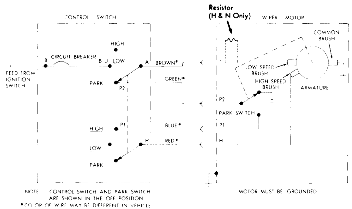
Chrysler Corp. Non-Concealed Wiper With 2-Speed Motor Windshield Wiper System Wiring Diagram
