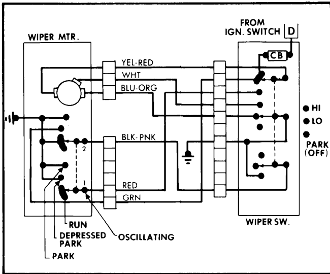
Cougar, Ford, Lincoln, LTD II, Mark V, Mercury, Rancho and Thunderbird 2-Speed Standard Depressed Windshield Wiper System Wiring Diagram
