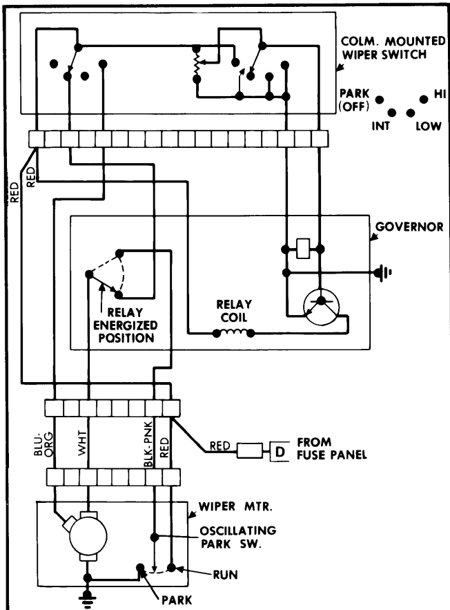
Fairmont, Granada, Monarch, Mustang, Versailles and Zephyr 2-Speed Intermittent Non-Depressed Windshield Wiper System Wiring Diagram
