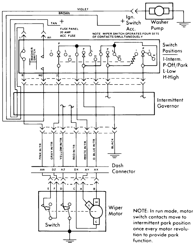
American Motors Matador Concealed Intermittent Windshield Wiper System Wiring Diagram
