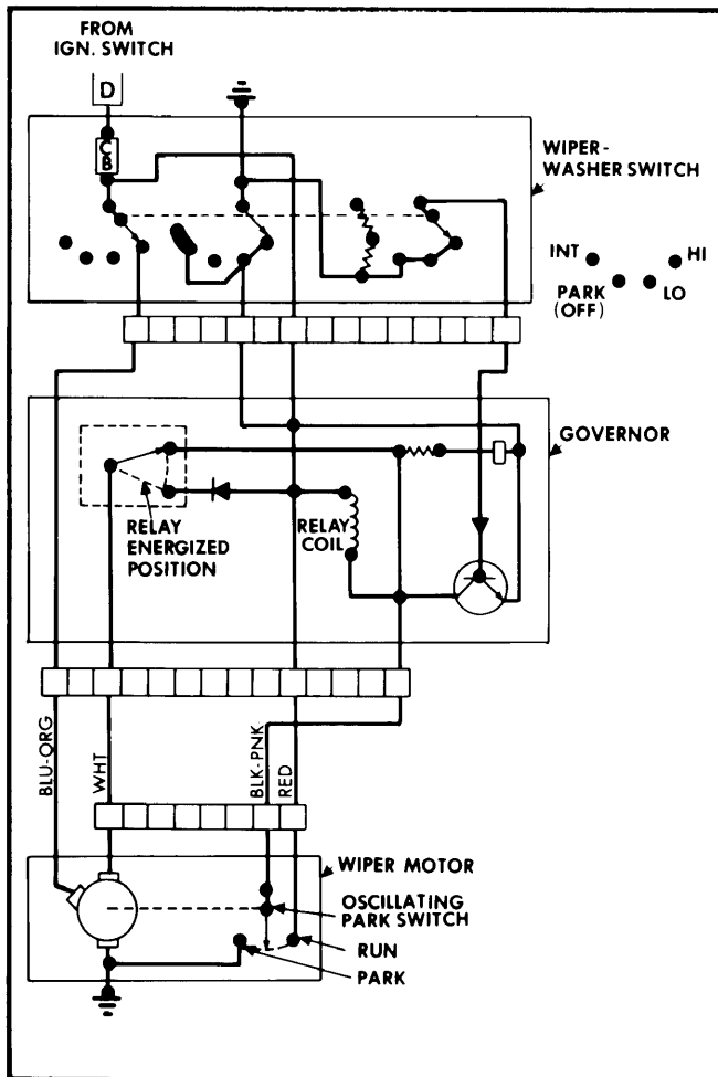
Pinto and Bobcat 2-Speed Standard Non-Depressed Windshield Wiper System Wiring Diagram
