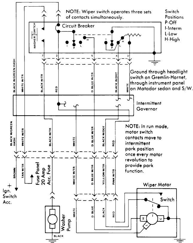
American Motors Non-Concealed Intermittent Windshield Wiper System Wiring Diagram
