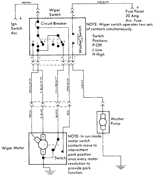
American Motors Non-Concealed Standard Windshield Wiper System Wiring Diagram
