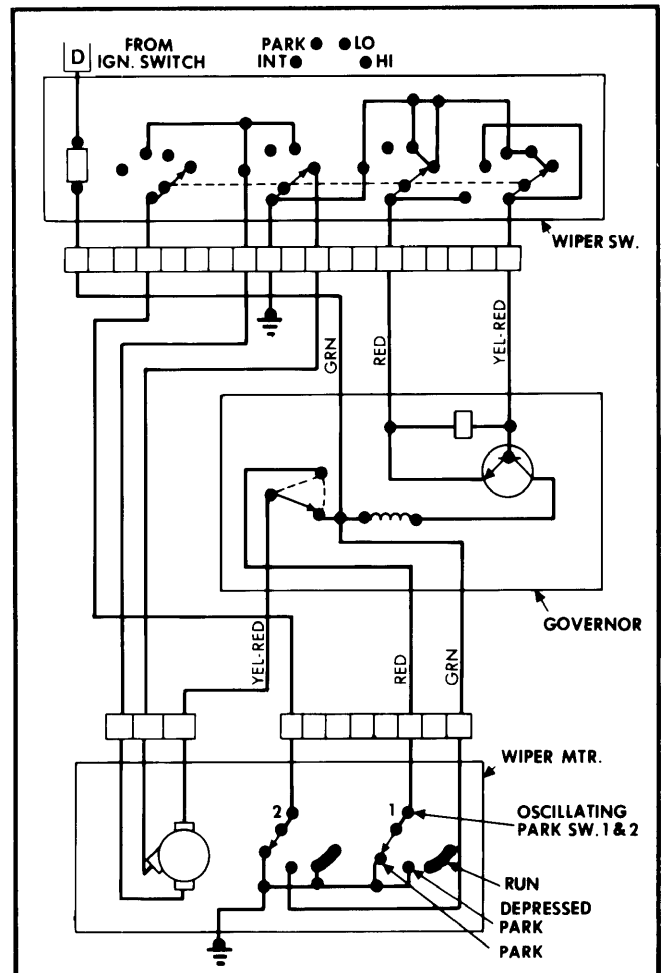
Cougar, Ford, Lincoln, LTD II, Thunderbird, Mercury, Rancho and Mark V 2-Speed Intermittent Depressed Windshield Wiper Wiring Diagram System
