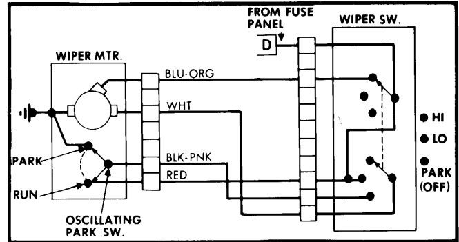
Pinto and Bobcat 2-Speed Intermittent Non-Depressed Windshield Wiper System Wiring Diagram
