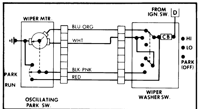
Fairmont, Granada, Monarch, Mustang, Versailles and Zephyr 2-Speed Standard Non-Depressed Windshield Wiper System Wiring Diagram
