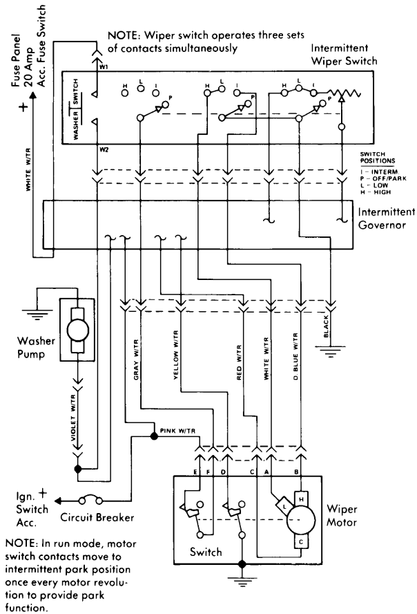
American Motors Pacer Concealed Intermittent Windshield Wiper System Wiring Diagram
