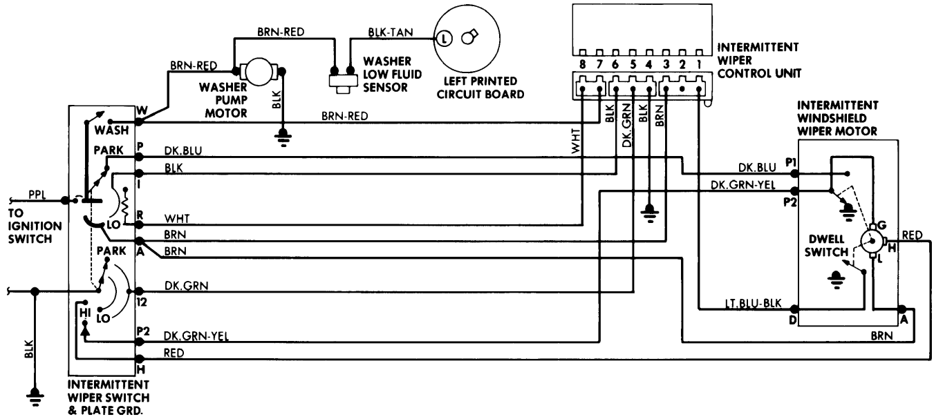
Chrysler Corp. 2-Speed Intermittent Windshield Wiper System Wiring Diagram
