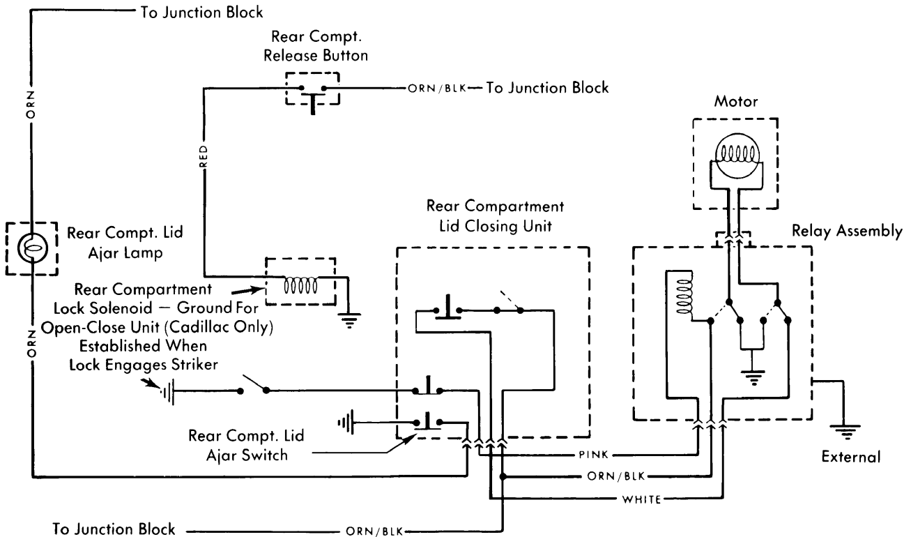
General Motors Electric Trunk Lid Latch Wiring Diagram Showing Cadillac Trunk Lid Opening and Closing Circuit
