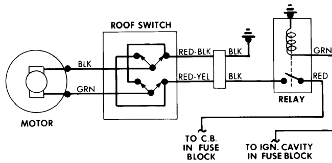
General Motors Sunroof Wiring Diagram (Buick Shown, Others Similar)
