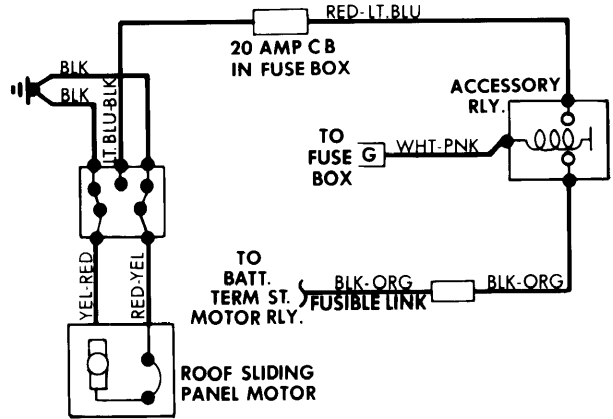
Ford Motor Co. Electric Sunroof Wiring Diagram
