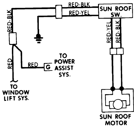
Chrysler Corp. Electric Sunroof Wiring Diagram
