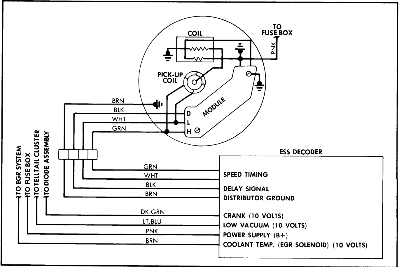
Cadillac Seville ESS Spark Timing System Schematic
