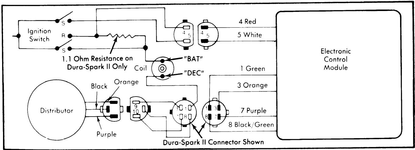
Ford Motor Co. Dura-Spark I and II Ignition System Wiring Diagram
