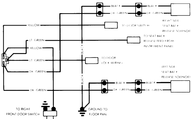
Chrysler Corp. Electric Seat Back Latch Wiring Diagram
