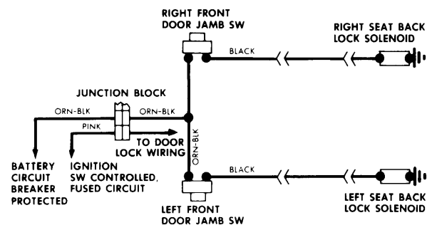
General Motors Electric Seat Back Latch Wiring Diagram
