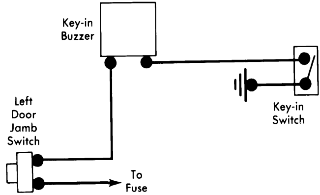
Ford Motor Co. Key Warning Buzzer Wiring Diagram
