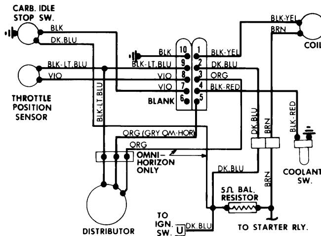
Chrysler Corp. Electronic Lean Burn System Wiring Diagram (Including Omni & Horizon)
