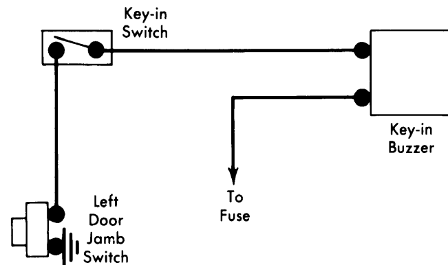
General Motors Separate Key Warning Buzzer Wiring Diagram (Buick, Chevrolet)
