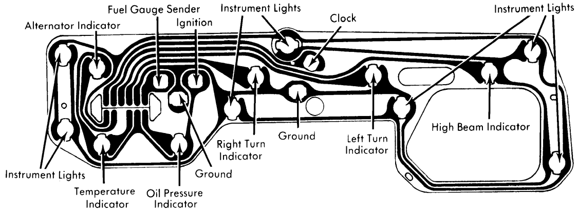
Catalina & Bonneville Instrument Cluster with Indicator Lights
