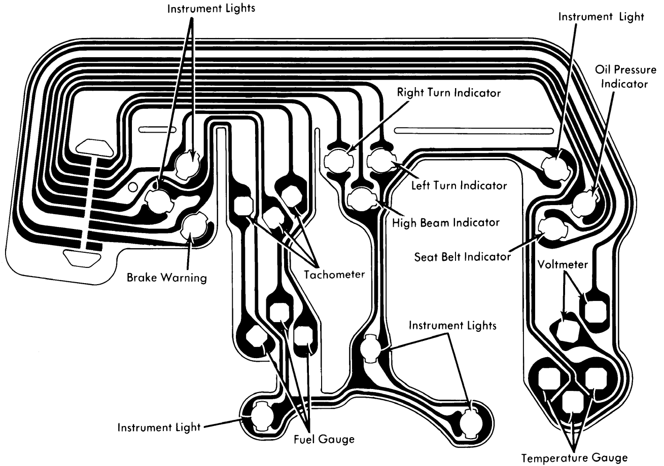
Sunbird Instrument Cluster with Gauges
