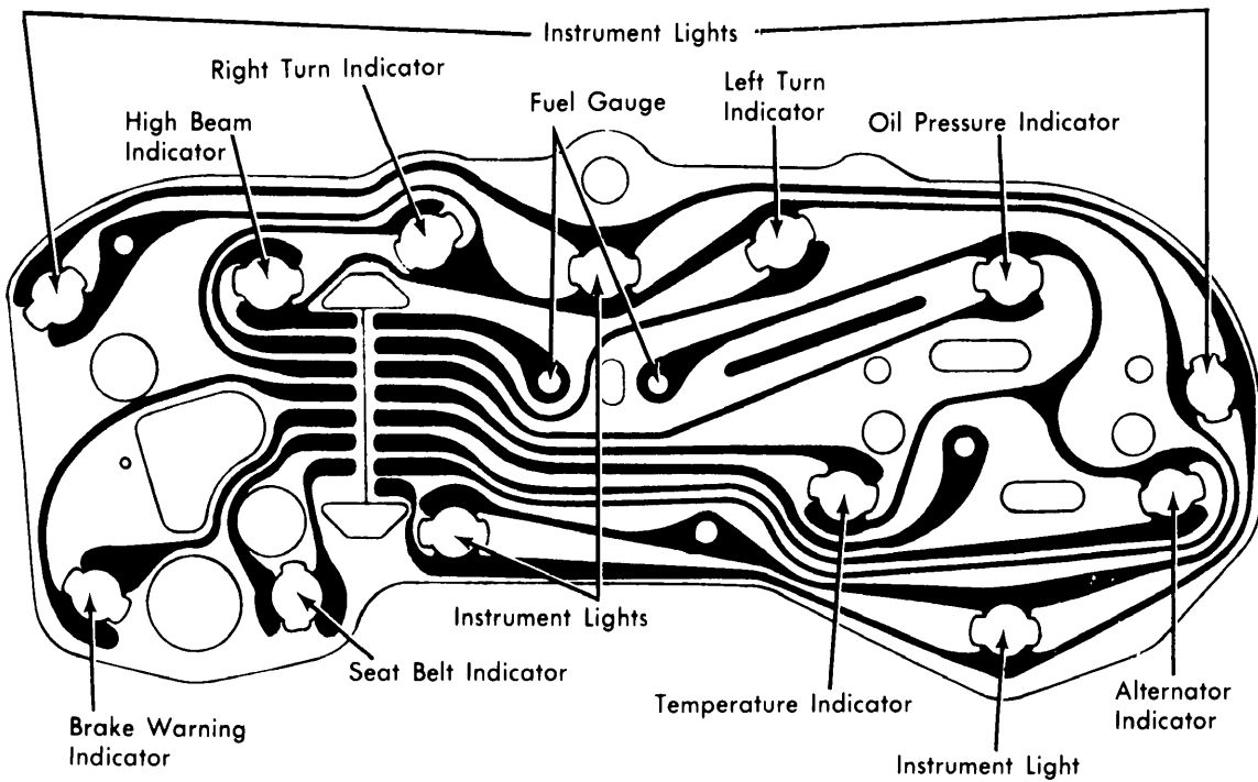
Firebird Instrument Cluster with Indicator Lights
