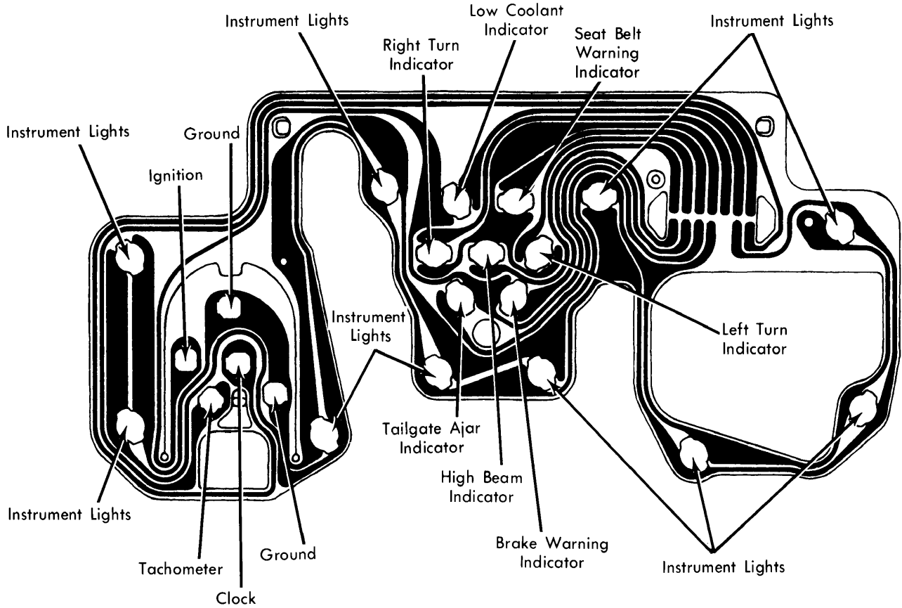
LeMans & Grand Prix Instrument Cluster
