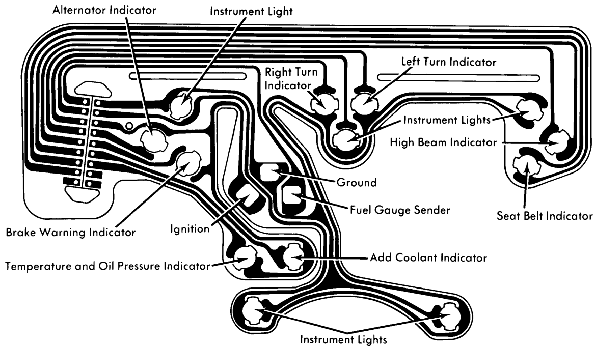
Starfire Instrument Cluster with Indicator Lights
