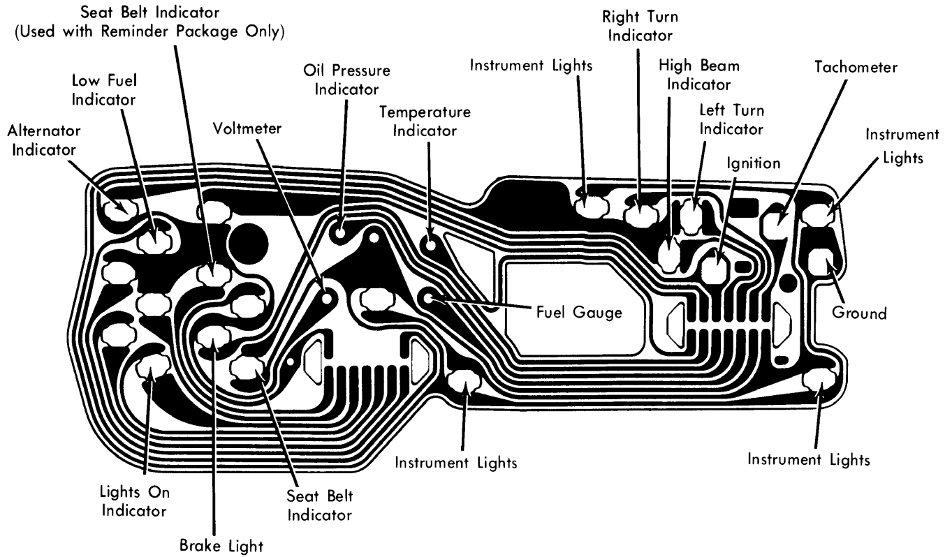
Cutlass Instrument Cluster with Gauges
