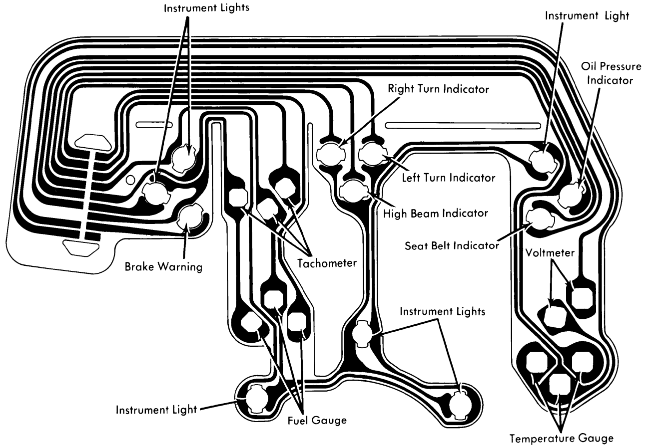
Starfire Instrument Cluster with Gauges
