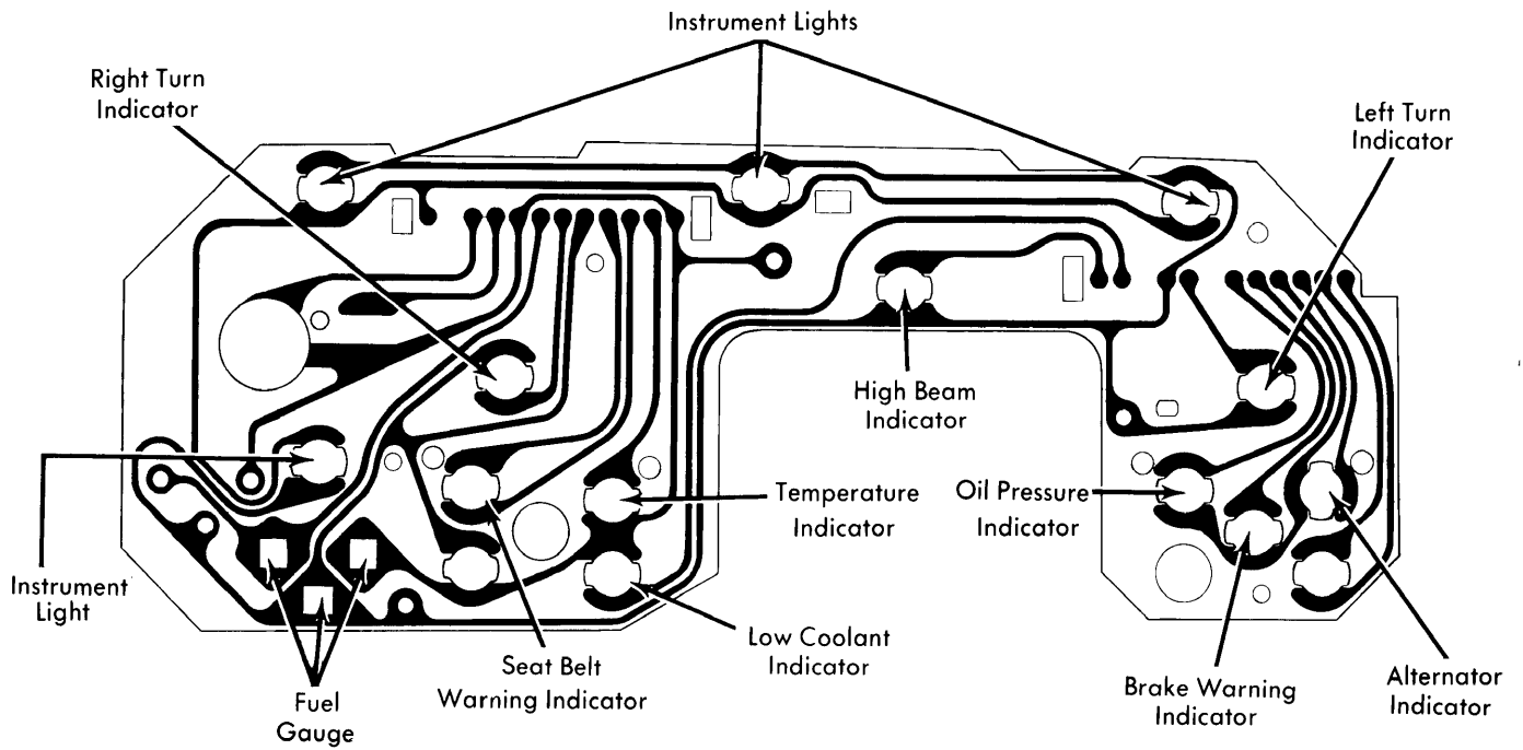
Toronado Instrument Cluster
