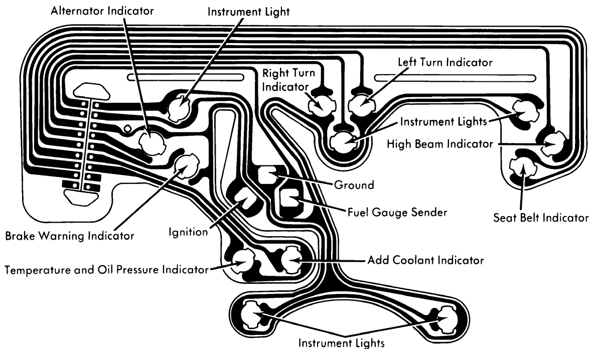
Sunbird Instrument Cluster with Indicator Lights
