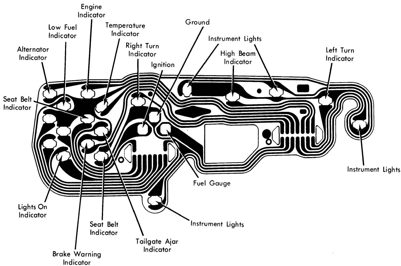
Cutlass Instrument Cluster without Gauges
