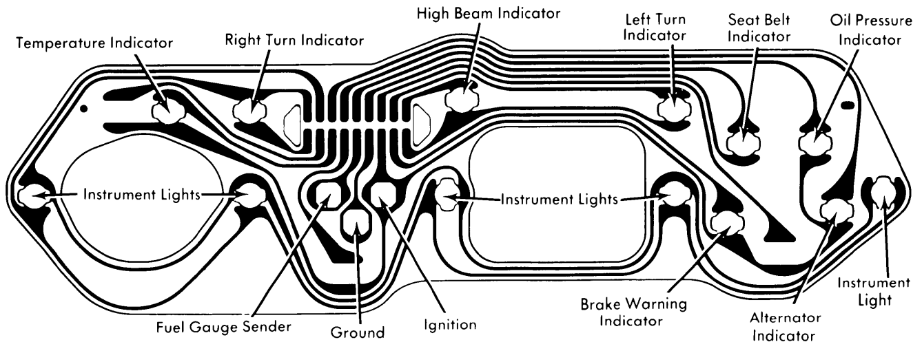
Omega Instrument Cluster with Indicator Lights
